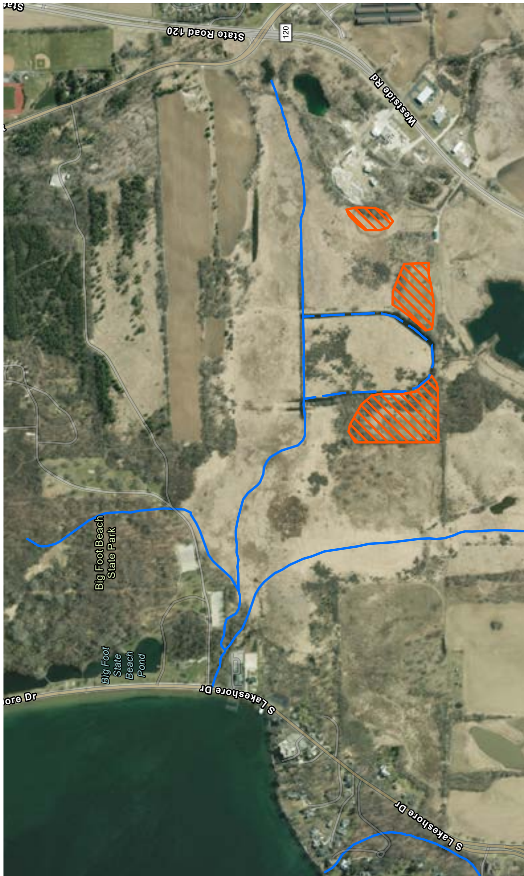
Map 2.21 Bigfoot Creek Mainstem, "Horseshoe," and Otto Jacobs Landfill Sites
