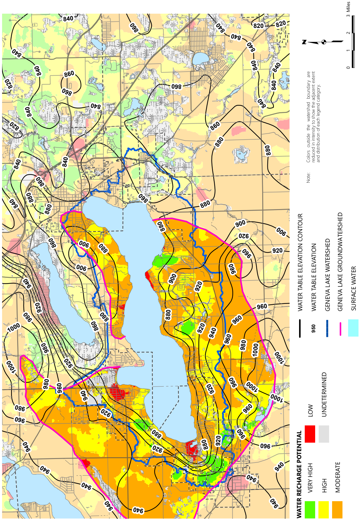
Figure A.3 Groundwater Elevation Contours and Recharge Potential Within and Beyond the Geneva Lake Watershed: SE Quadrant
