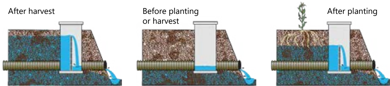
Figure 3.6 Inline Water Control Diagram
