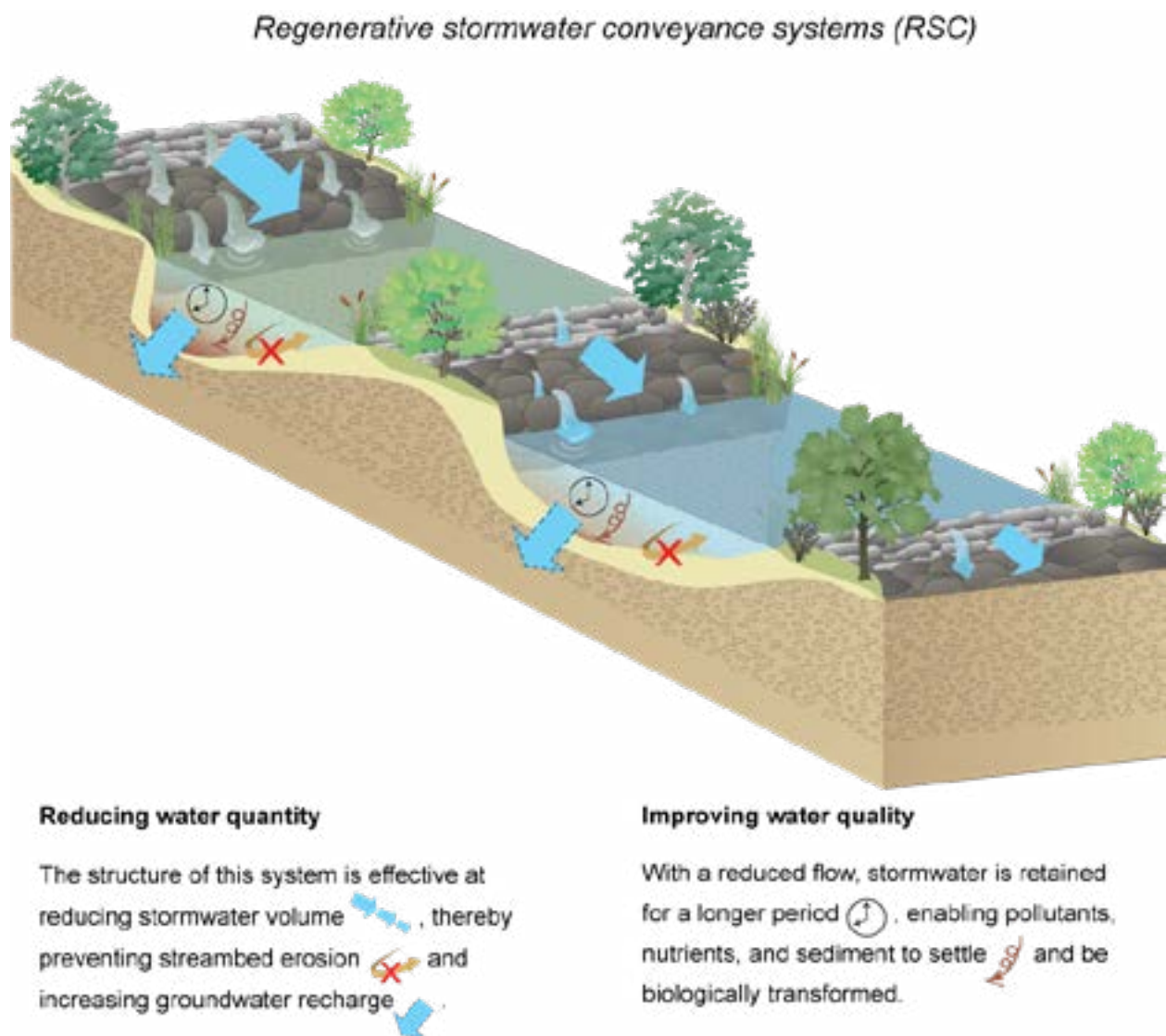
Figure 3.7 Regenerative Stormwater Conveyance
