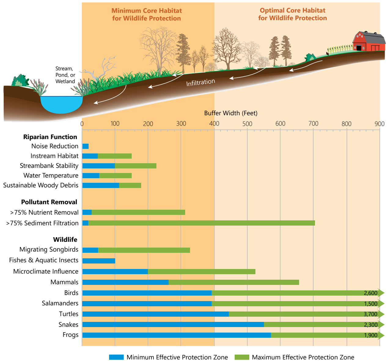
Figure 3.10 Shoreline Buffer Benefits
