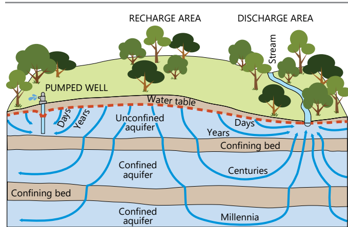
Figure 2.6 Regional vs. Local Groundwater Flow Paths
