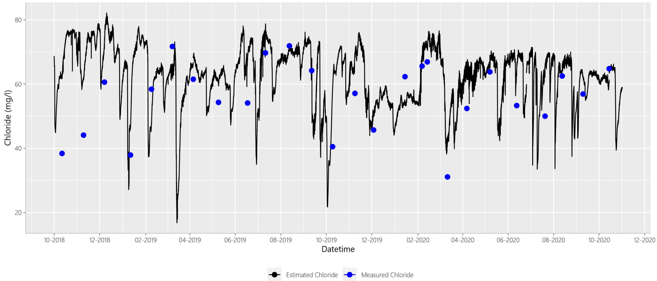
Figure A.Site28ClEstClTimeSeries
