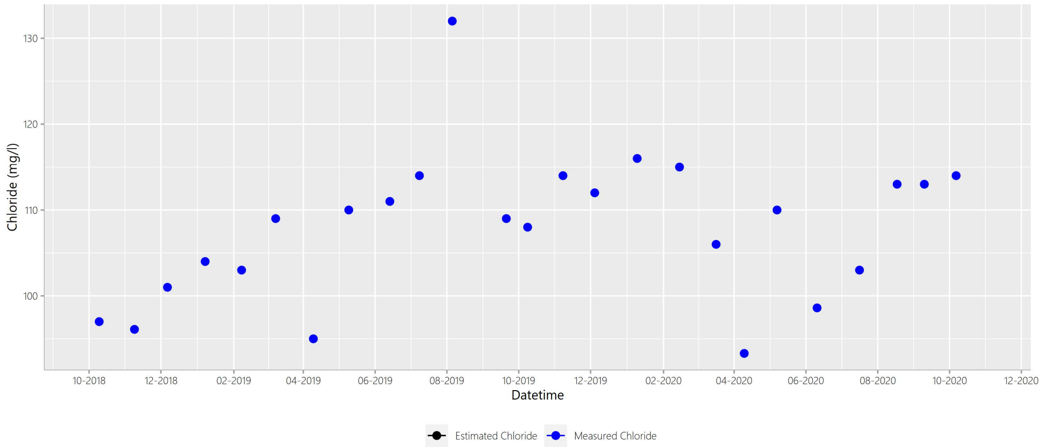
Figure A.Site55ClEstCITimeSeries
