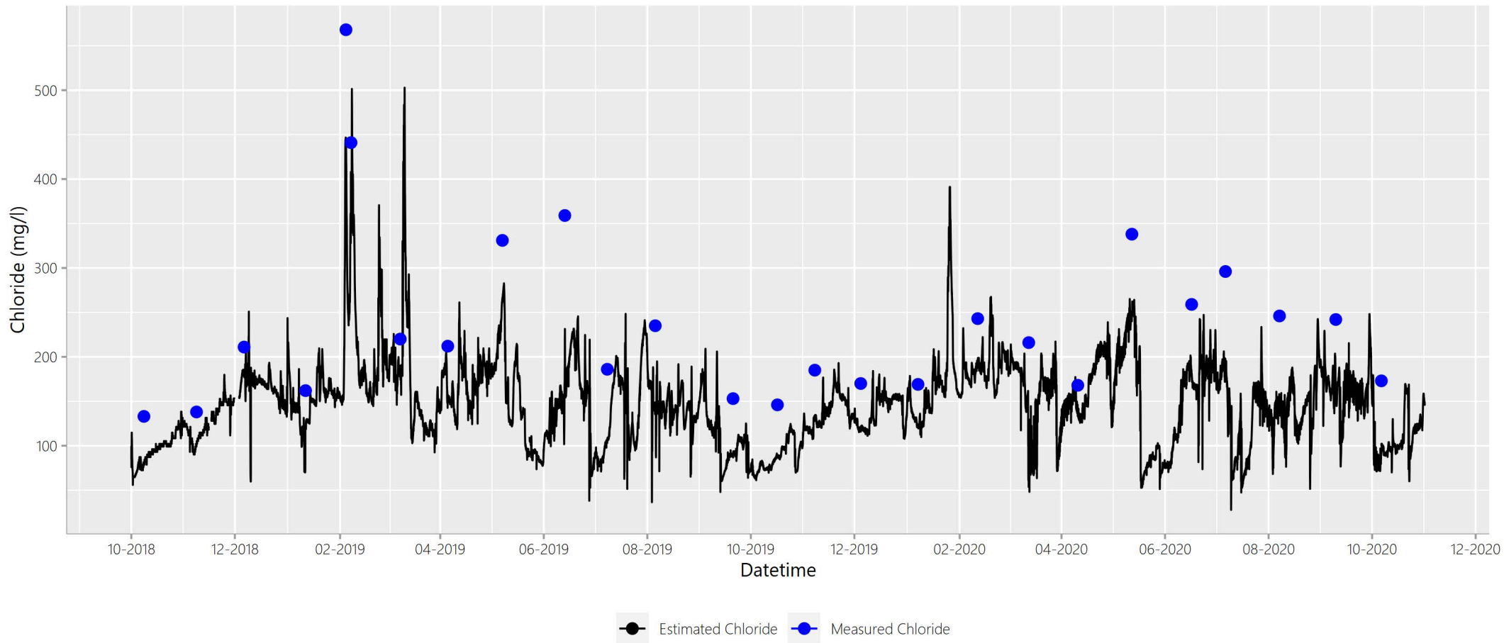
Figure A.Site08ClEstClTimeSeries
