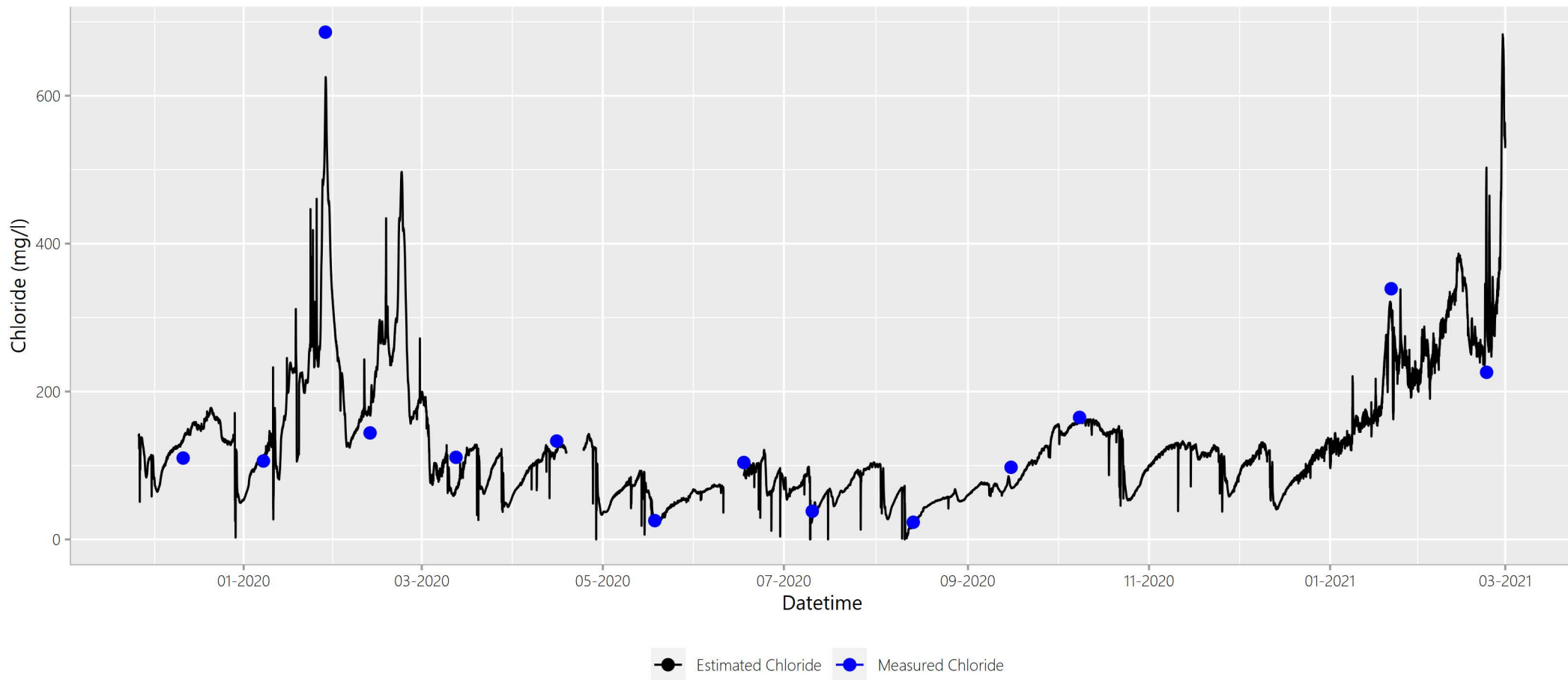
Figure A.Site59ClEstCITimeSeries
