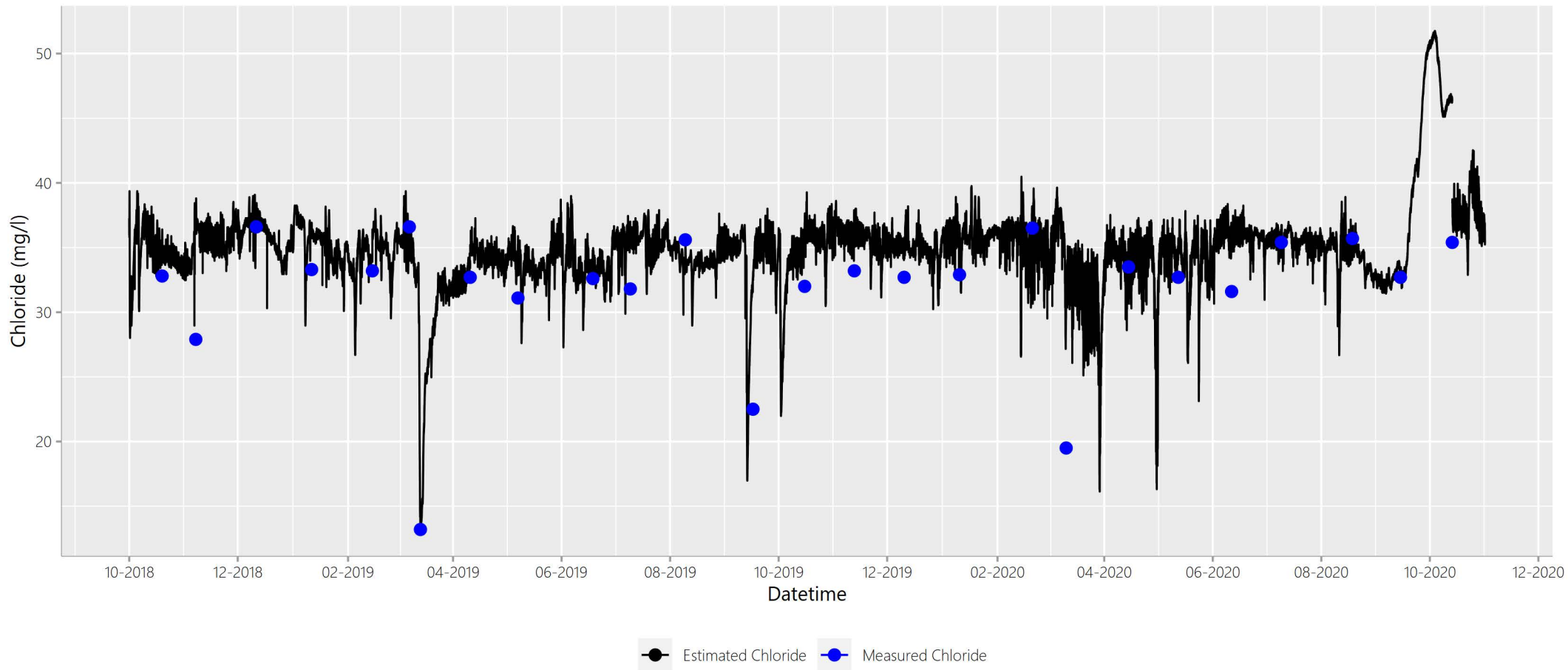
Figure A.Site35ClEstClTimeSeries
