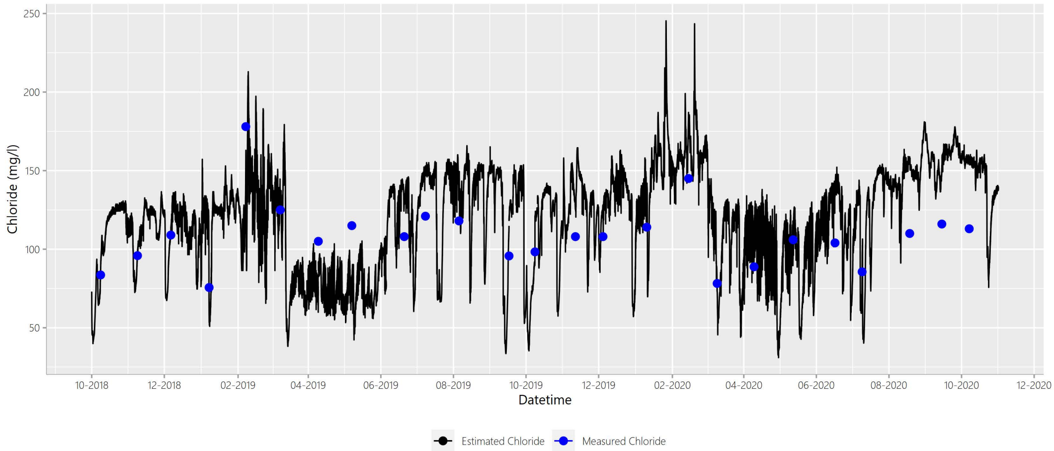
Figure A.Site33ClEstCITimeSeries
