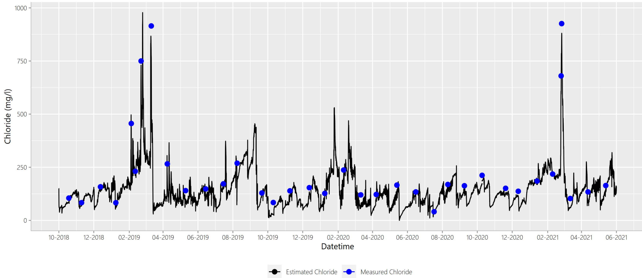
Figure A.Site13ClEstClTimeSeries
