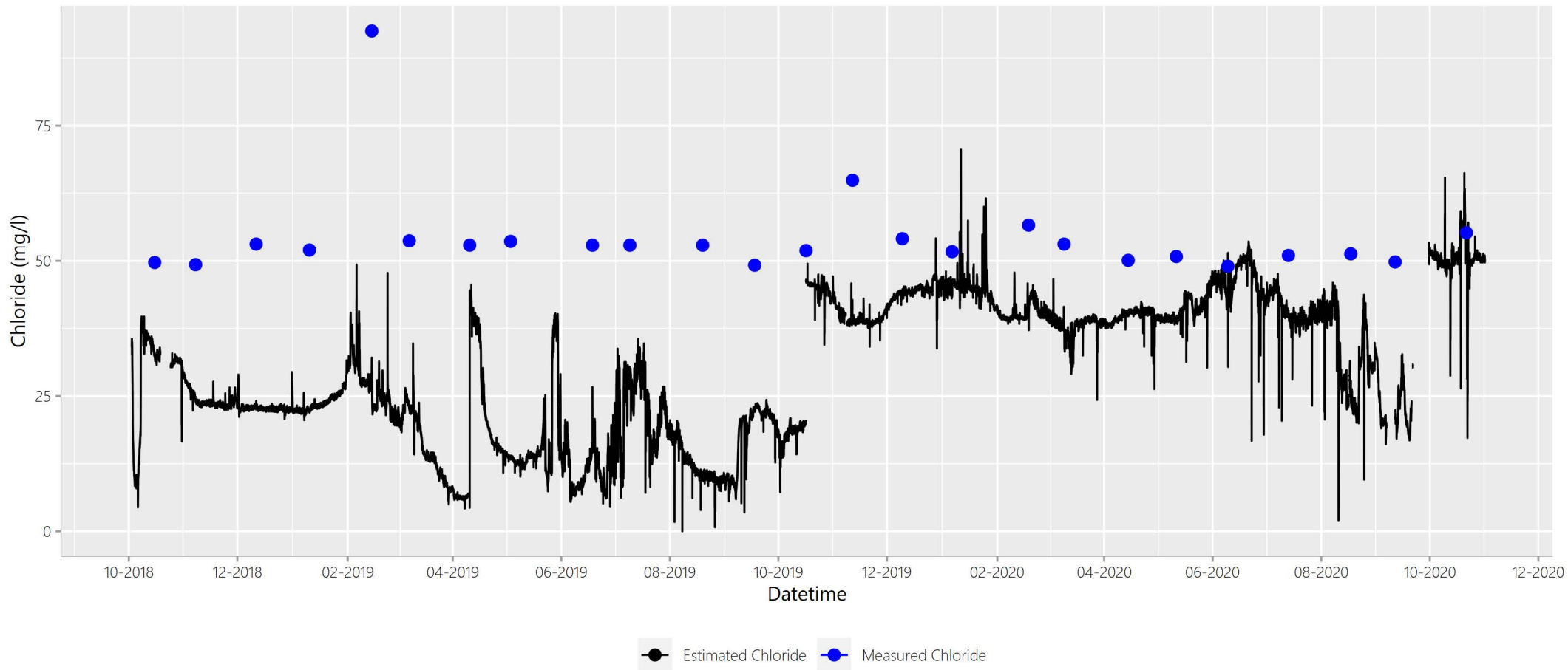
Figure A.Site48ClEstClTimeSeries
