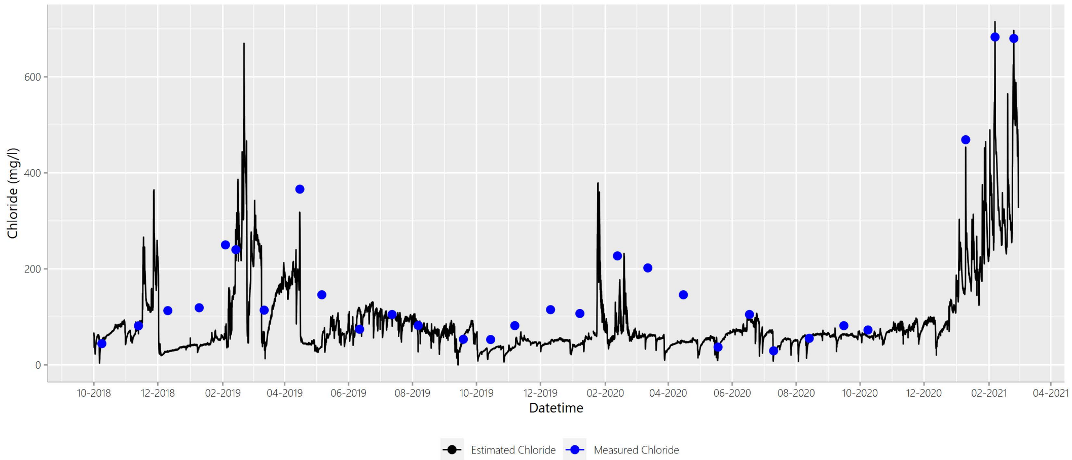
Figure A.Site10ClEstCITimeSeries
