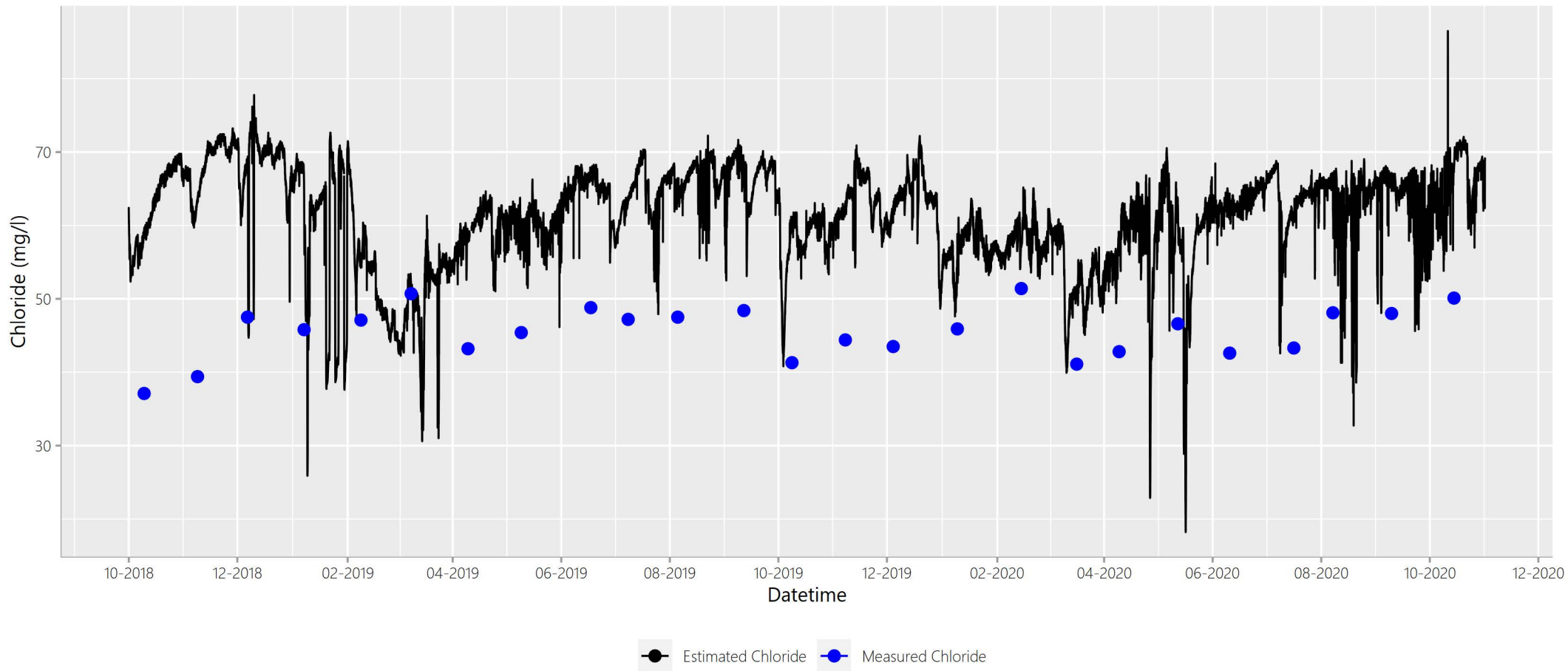
Figure A.Site18ClEstClTimeSeries
