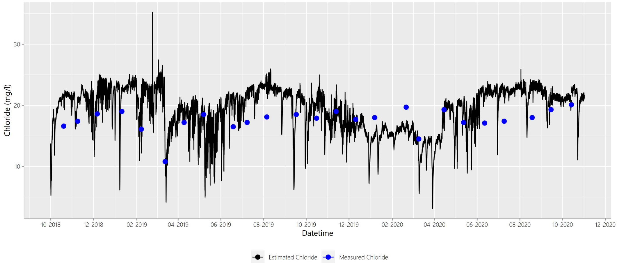
Figure A.Site45ClEstClTimeSeries
