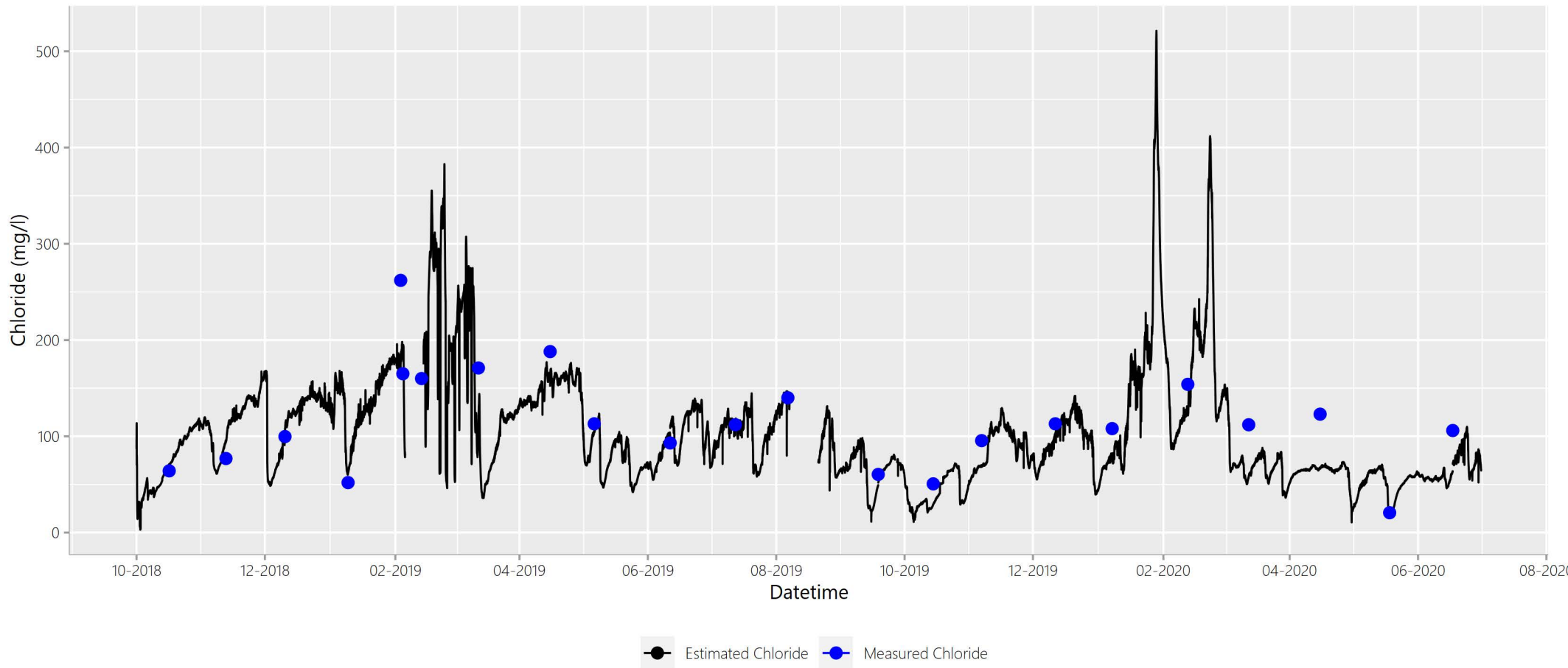
Figure A.Site29ClEstCITimeSeries
