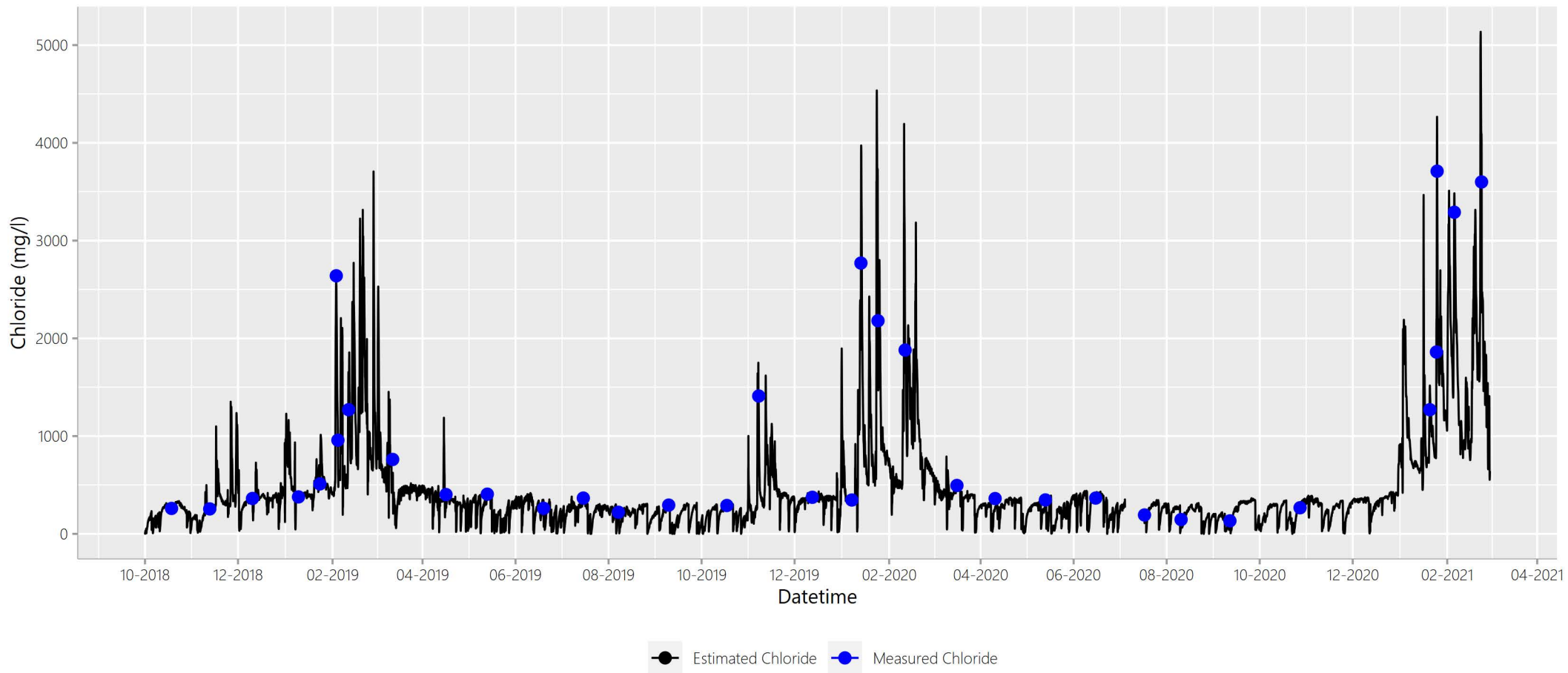
Figure A.Site12ClEstCITimeSeries
