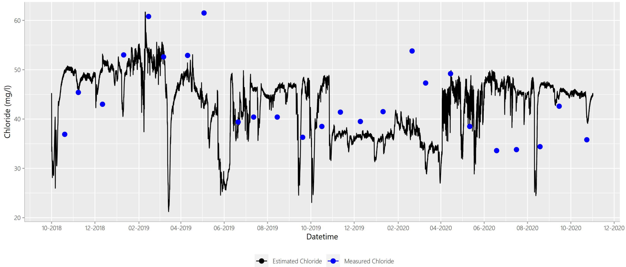
Figure A.Site04ClEstClTimeSeries
