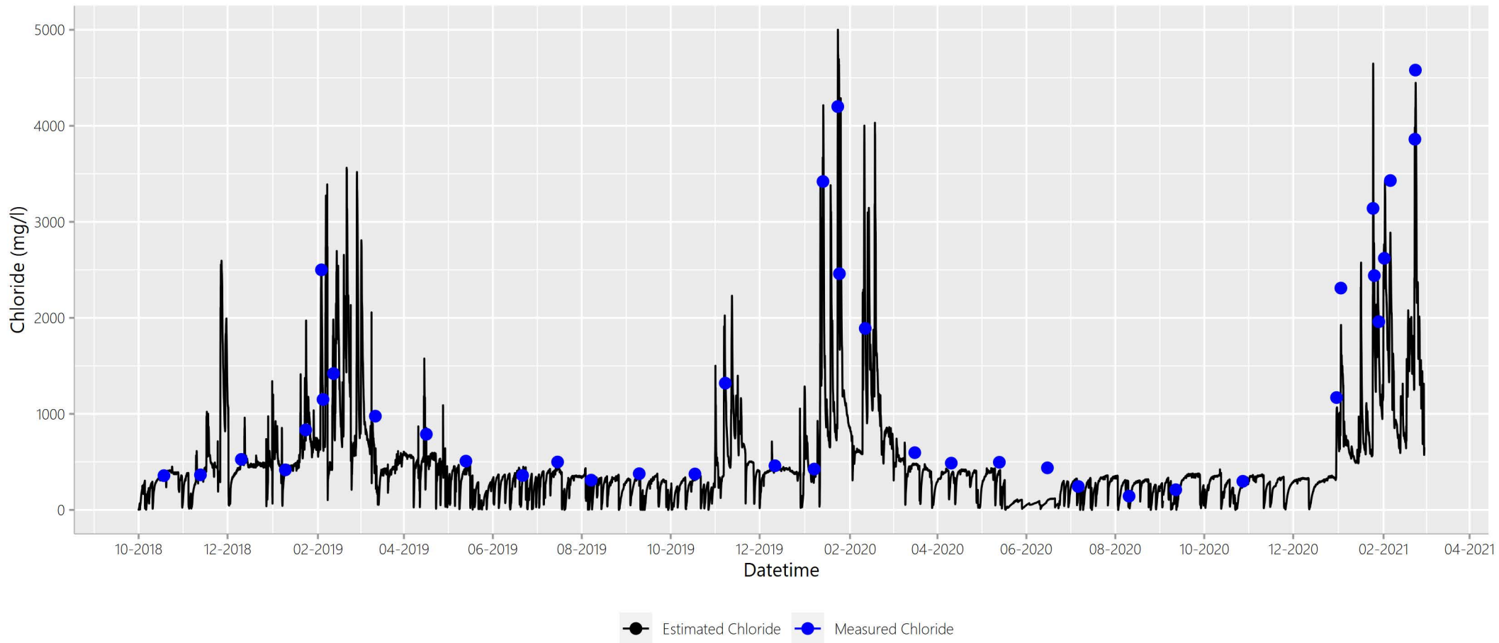
Figure A.Site53ClEstCITimeSeries
