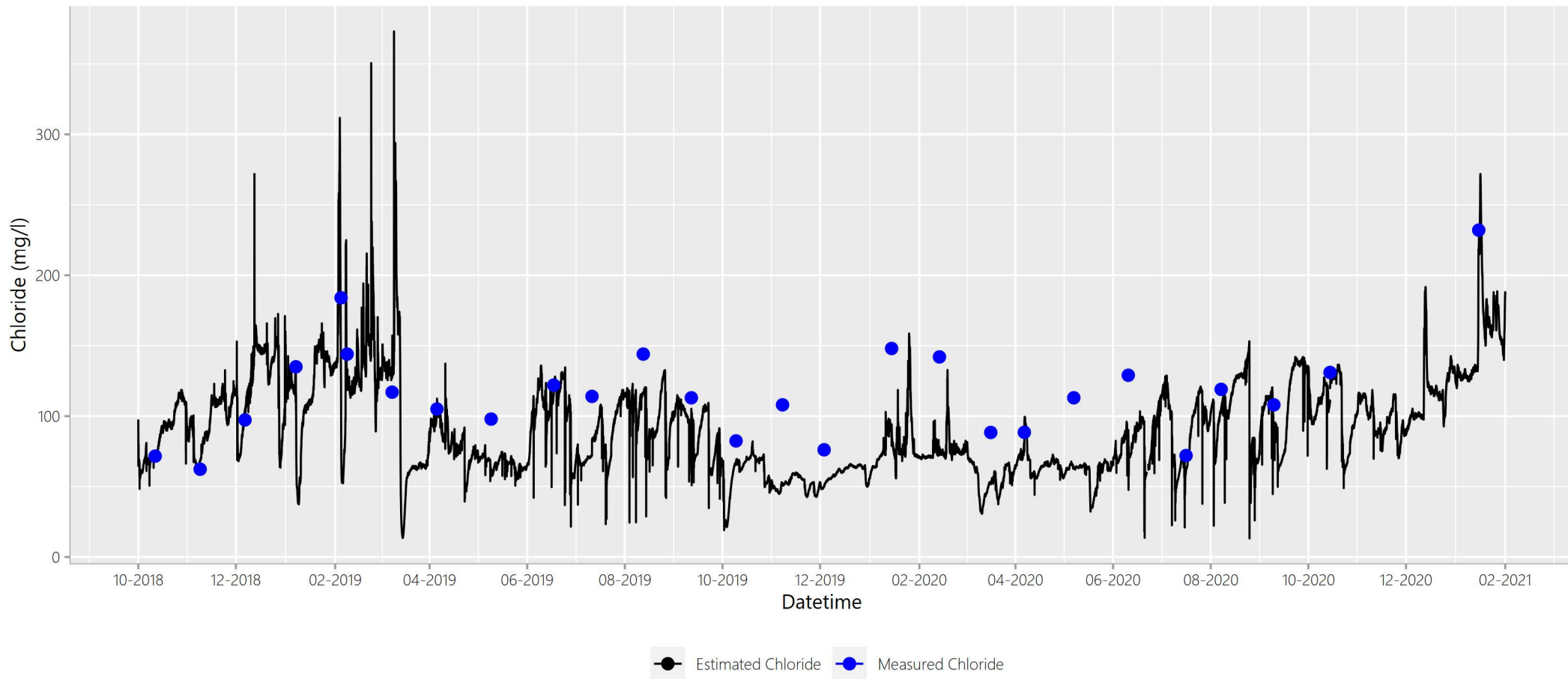
Figure A.Site51ClEstClTimeSeries
