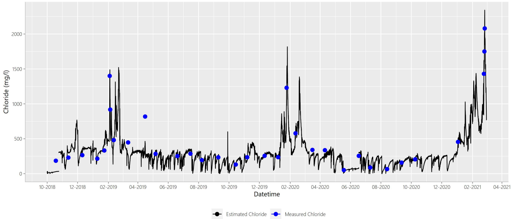
Figure A.Site09ClEstCITimeSeries
