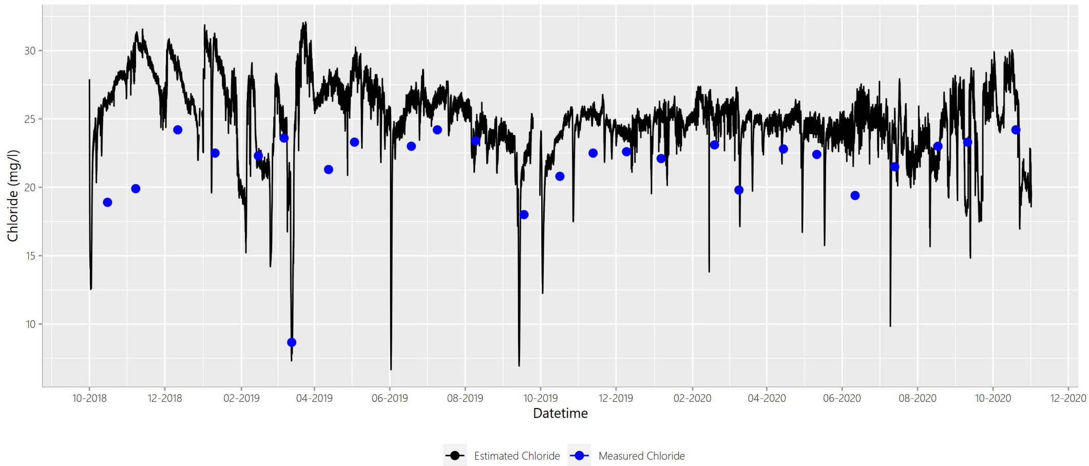
Figure A.Site54ClEstClTimeSeries
