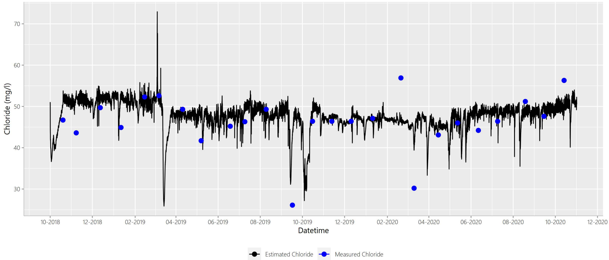
Figure A.Site36ClEstClTimeSeries
