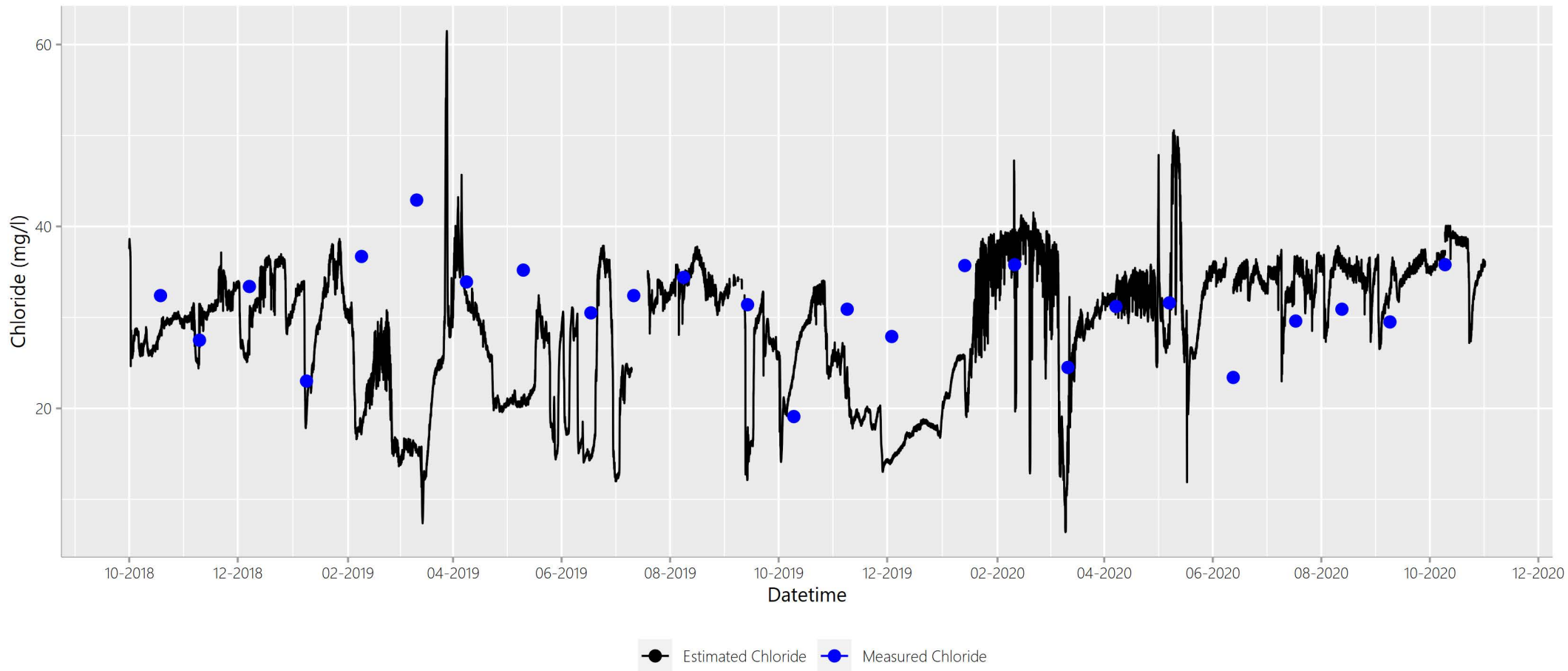
Figure A.Site40ClEstClTimeSeries
