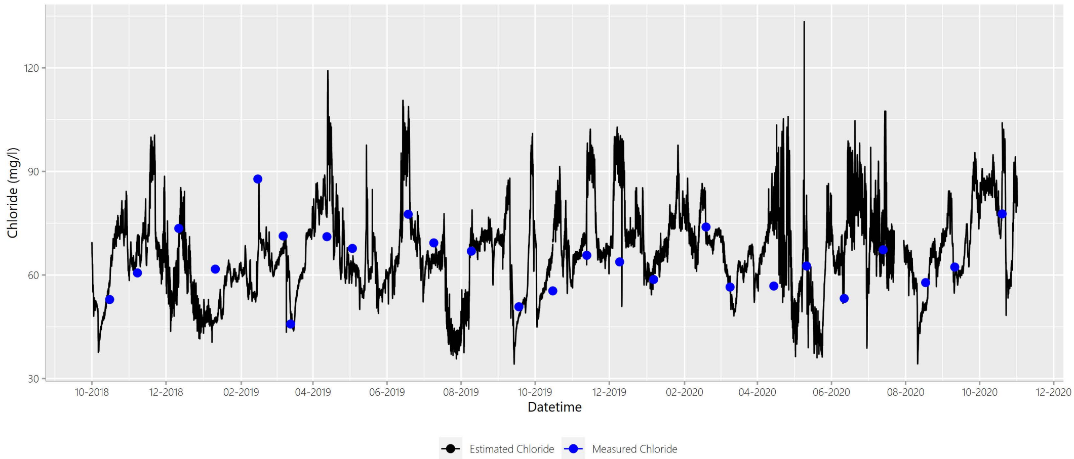
Figure A.Site32ClEstCITimeSeries
