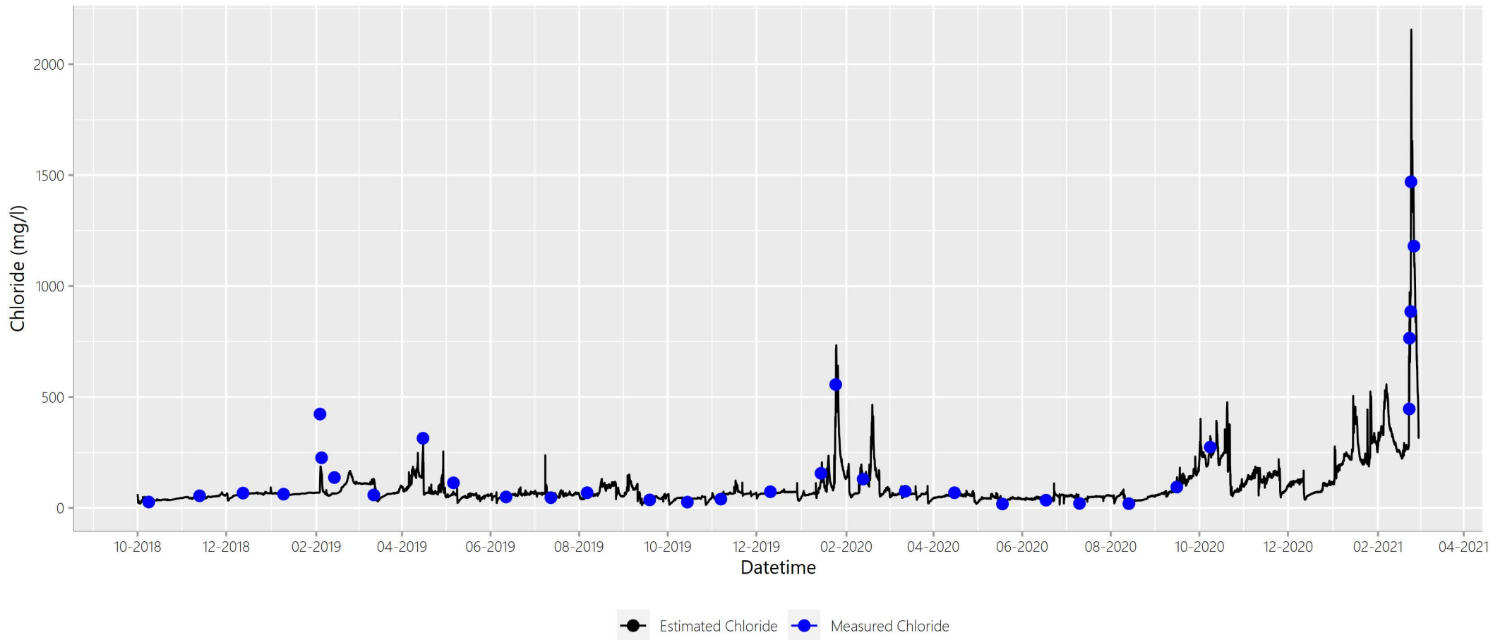
Figure A.Site15ClEstClTimeSeries
