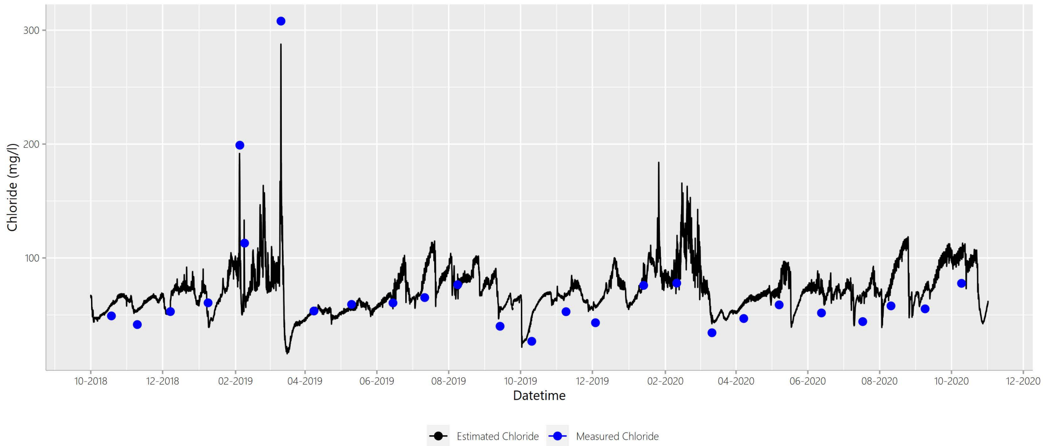
Figure A.Site23ClEstCITimeSeries
