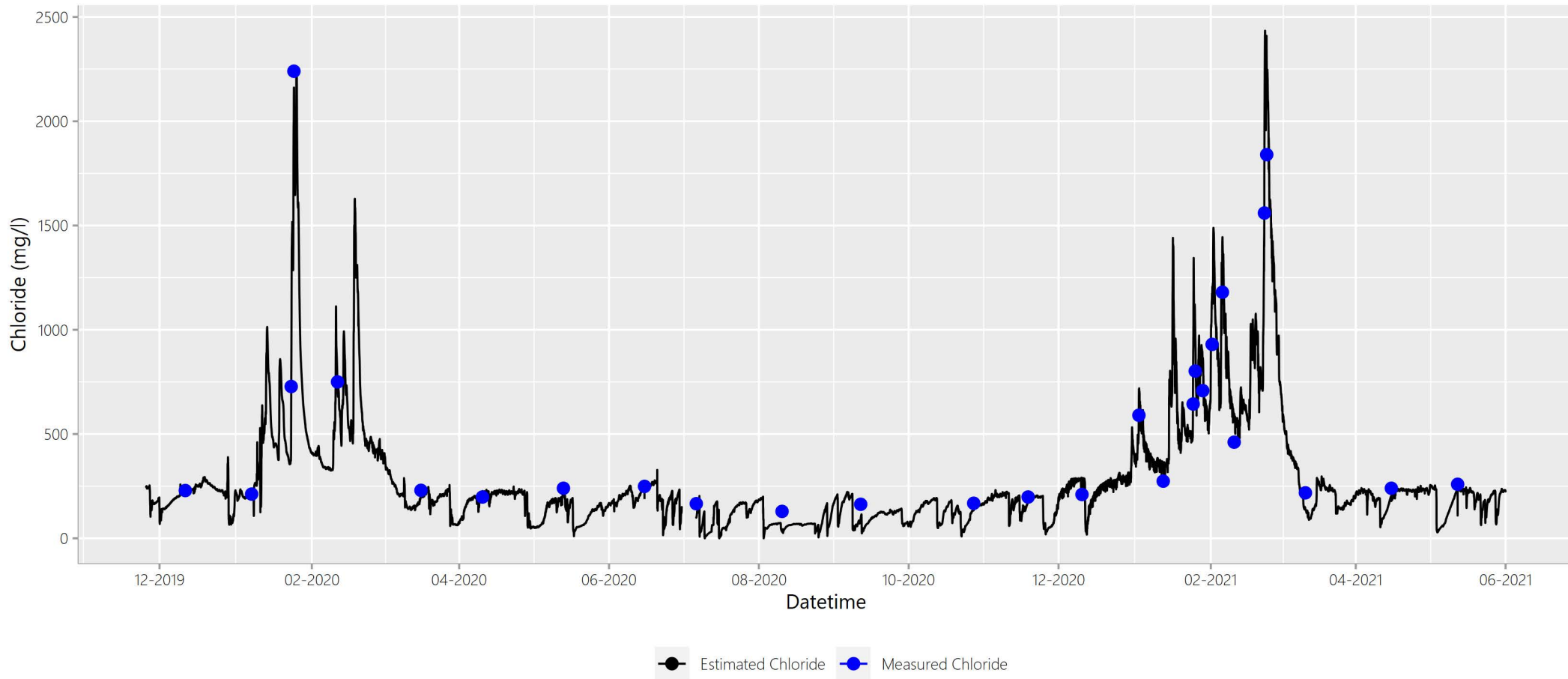
Figure A.Site57ClEstCITimeSeries
