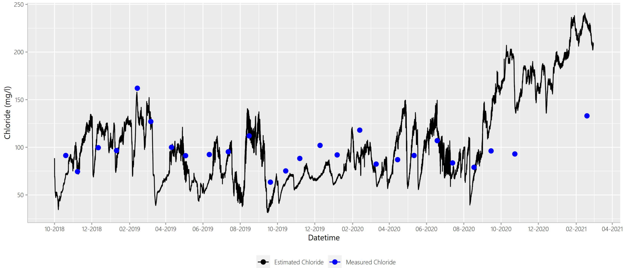
Figure A.Site02ClEstClTimeSeries
