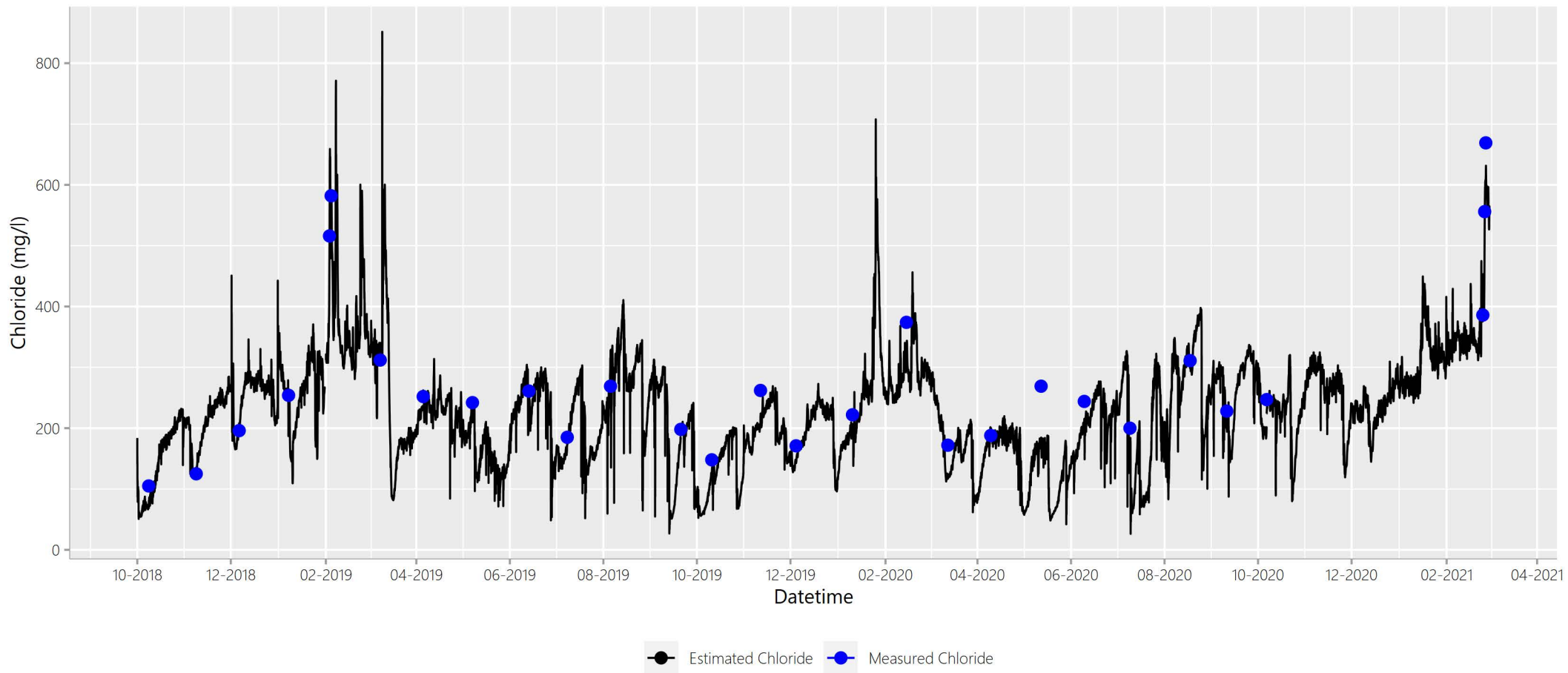
Figure A.Site01ClEstClTimeSeries
