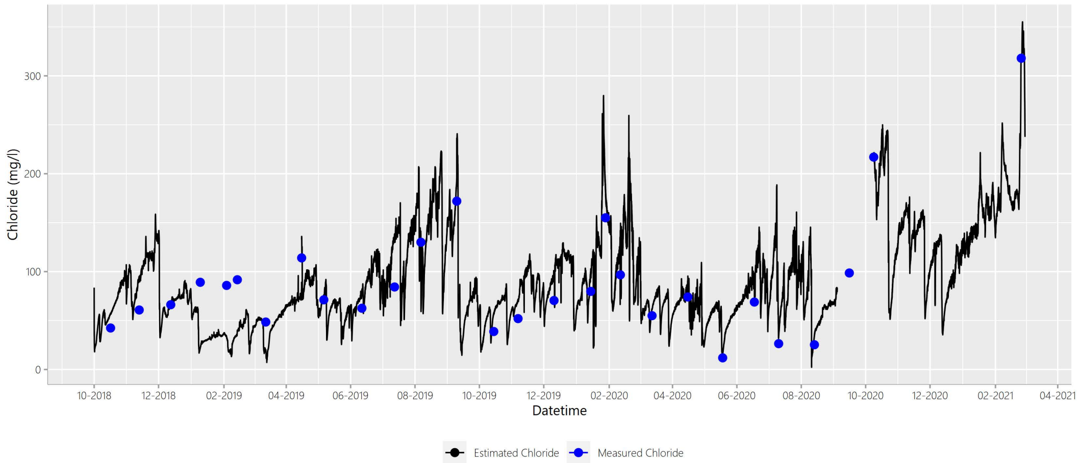
Figure A.Site25ClEstCITimeSeries
