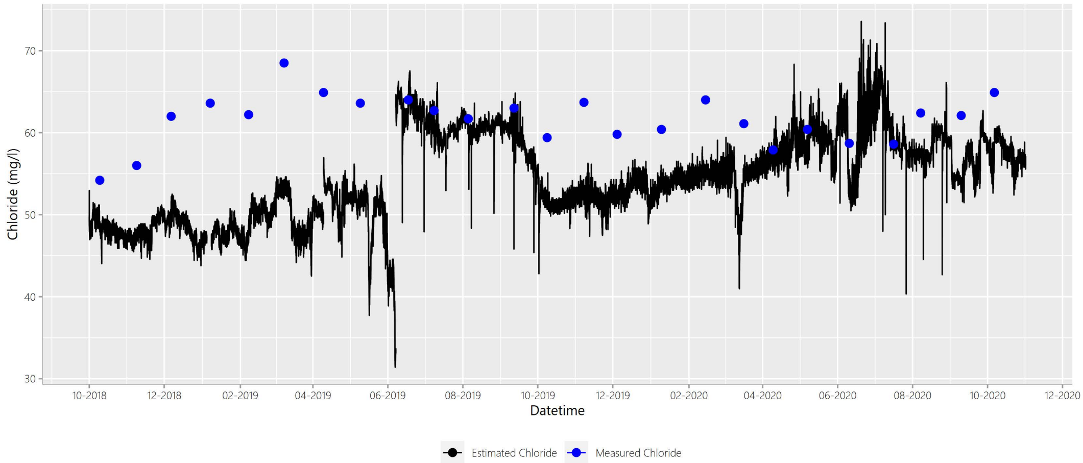
Figure A.Site20CIEstClTimeSeries
