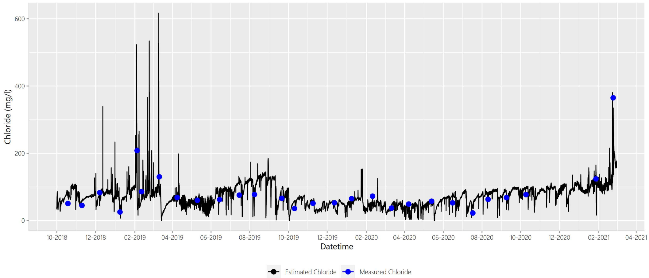
Figure A.Site14ClEstClTimeSeries
