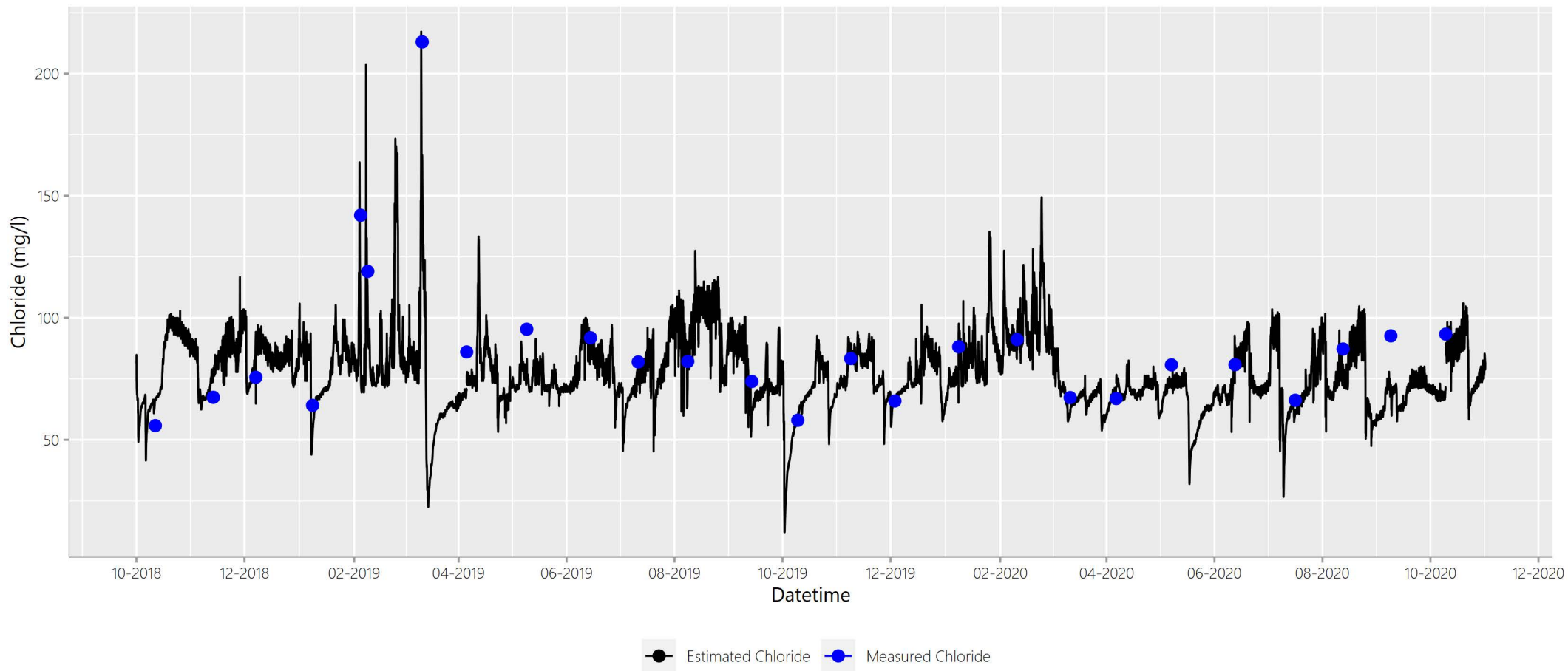
Figure A.Site52ClEstCITimeSeries
