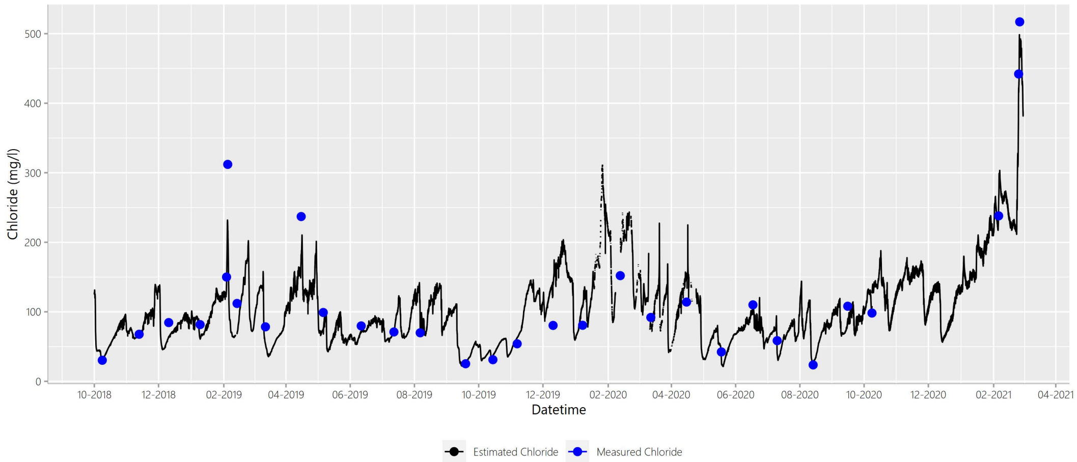
Figure A.Site30ClEstCITimeSeries
