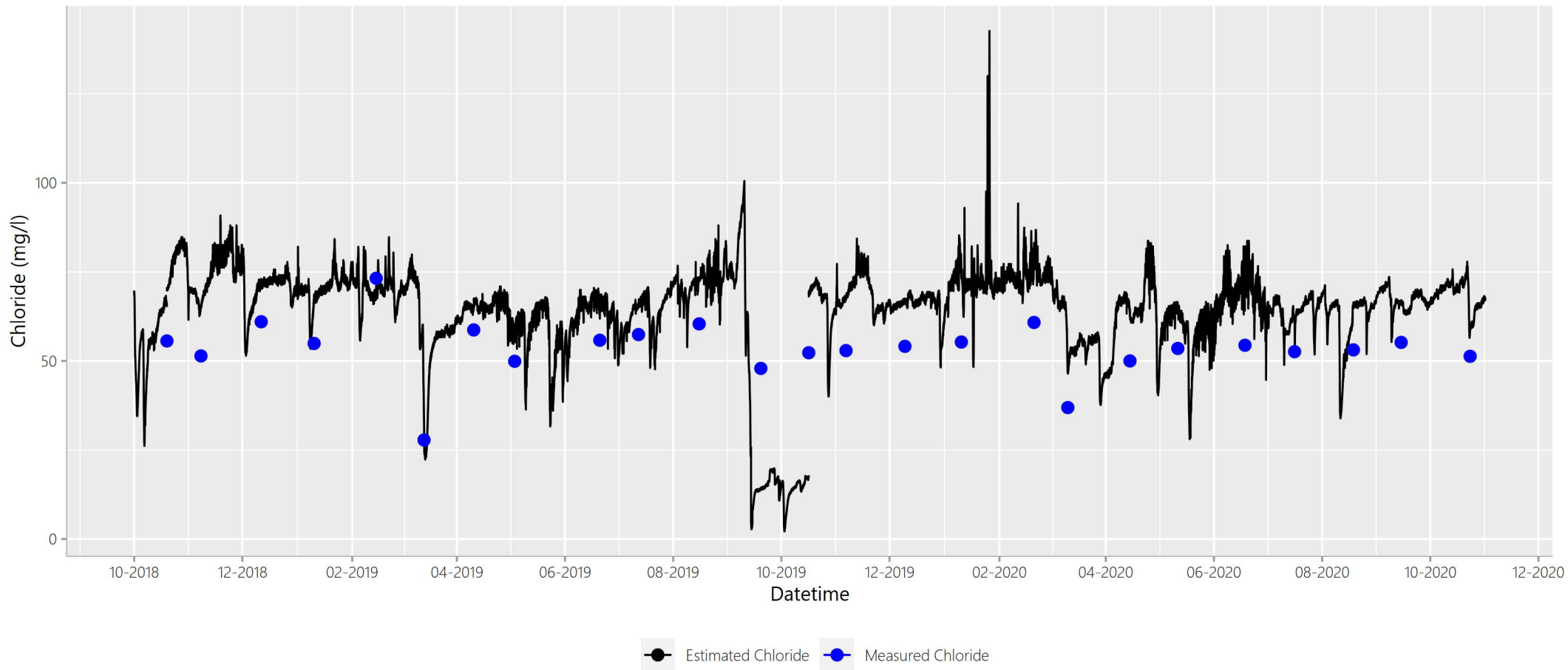
Figure A.Site06ClEstClTimeSeries
