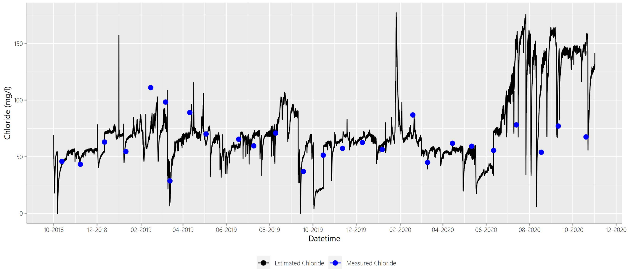
Figure A.Site16ClEstCITimeSeries
