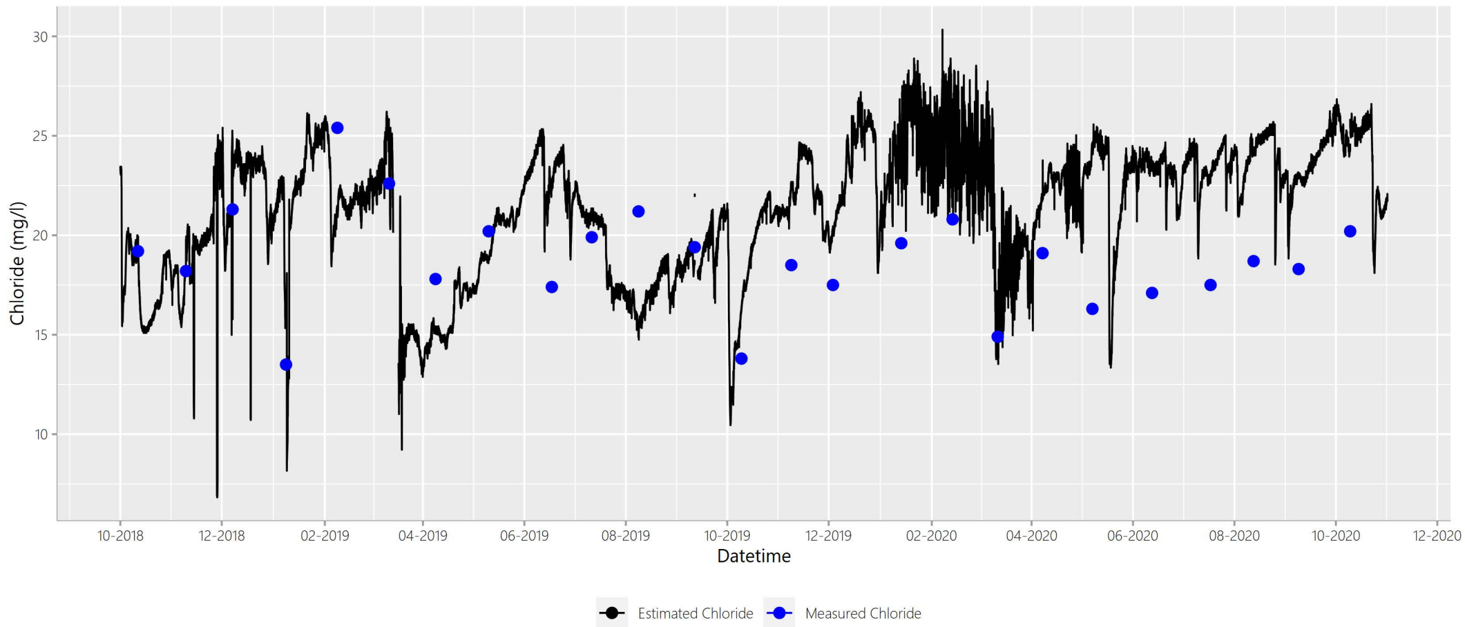
Figure A.Site21ClEstClTimeSeries
