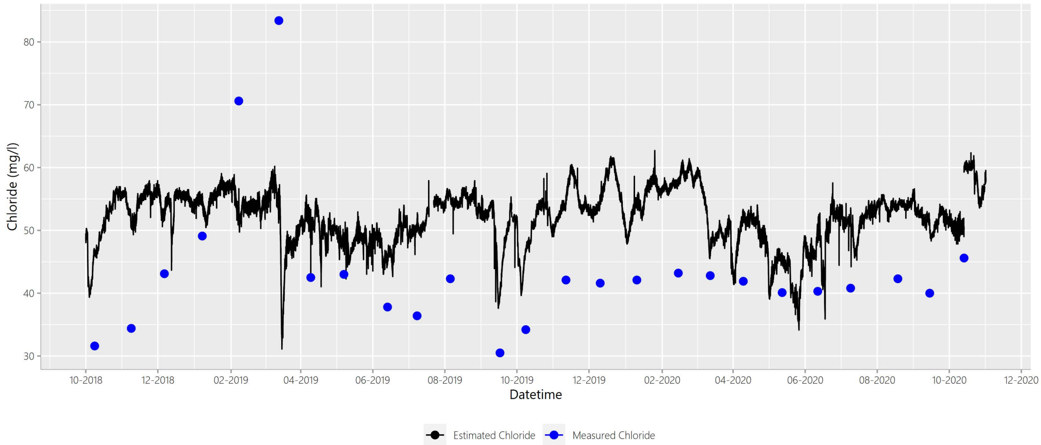
Figure A.Site03ClEstClTimeSeries
