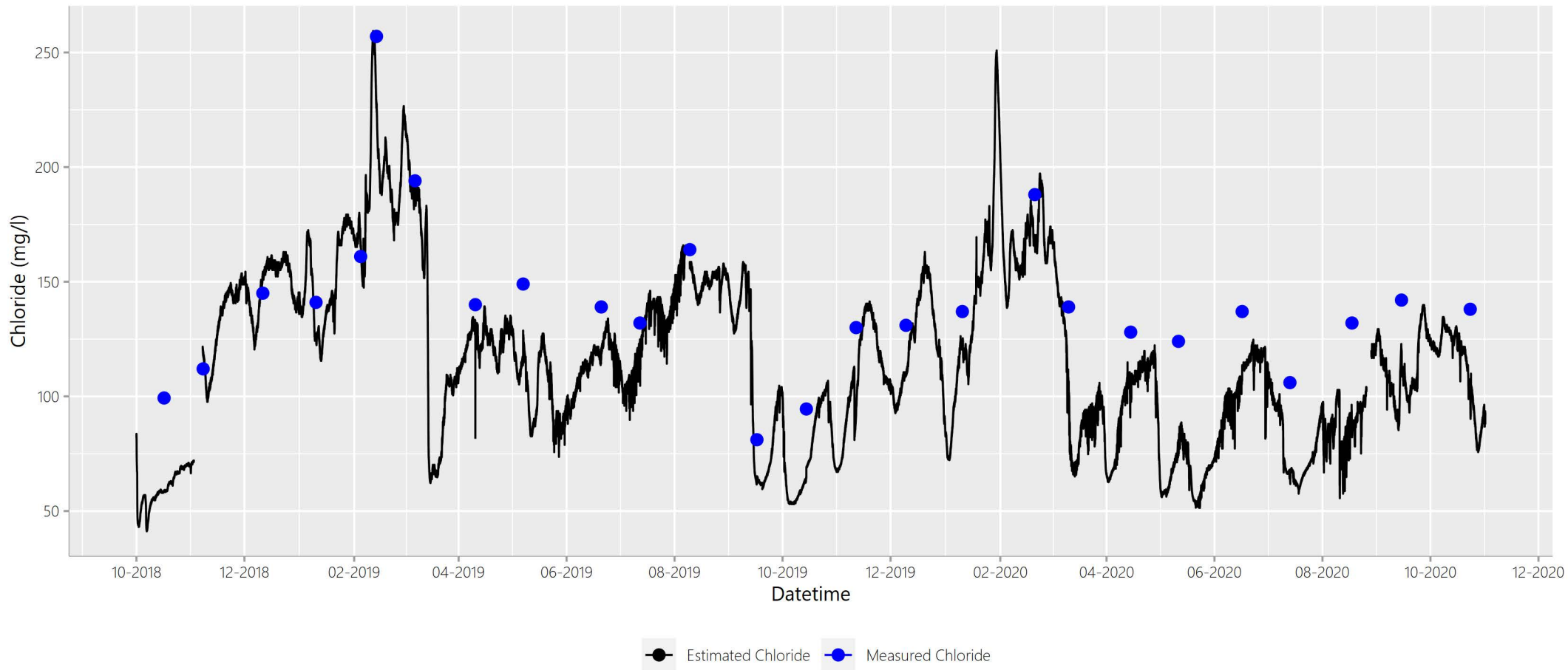
Figure A.Site47ClEstCITimeSeries
