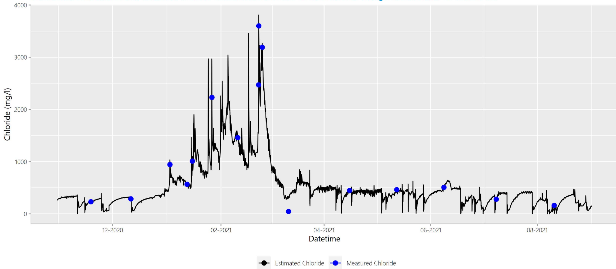
Figure A.Site60CIEstCITimeSeries
