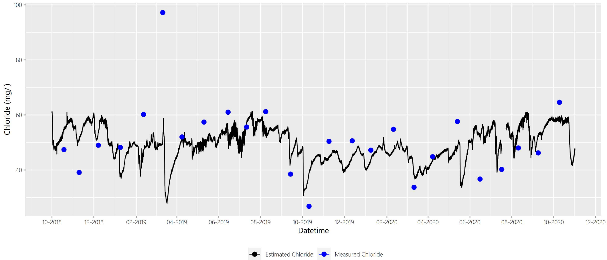
Figure A.Site41ClEstCITimeSeries
