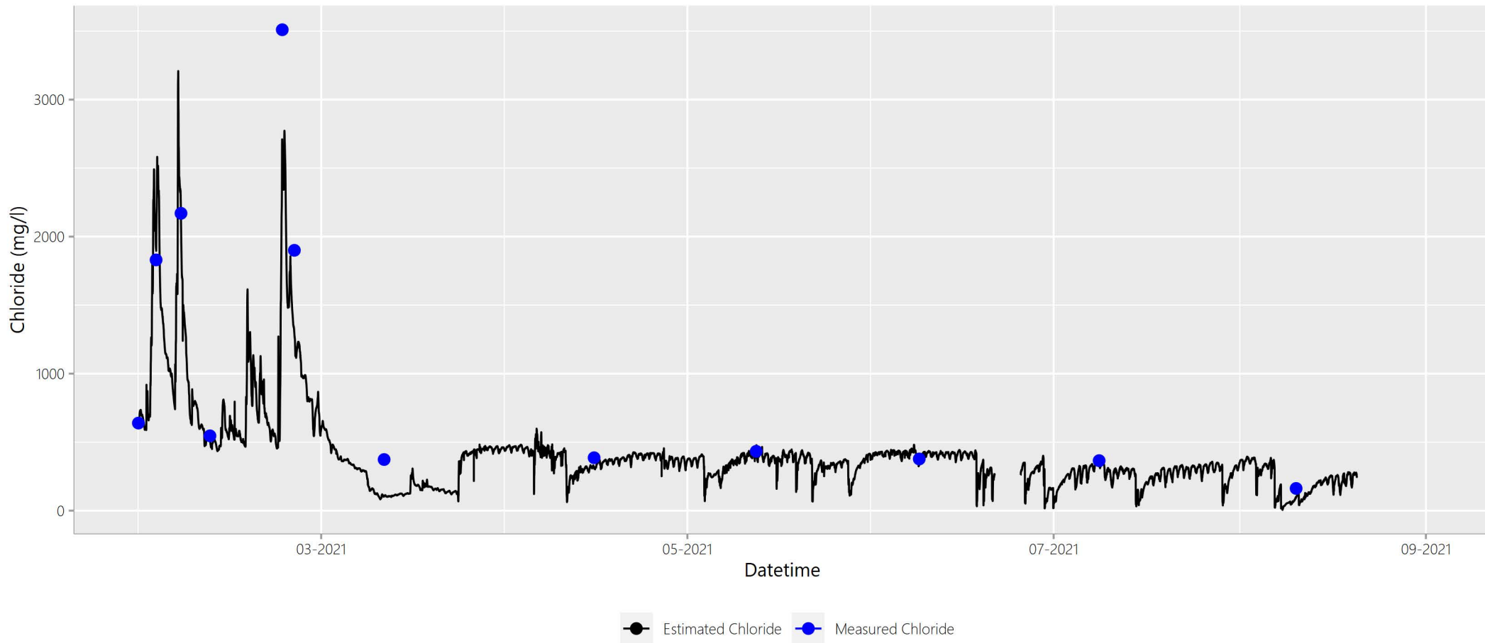
Figure A.Site87ClEstCITimeSeries
