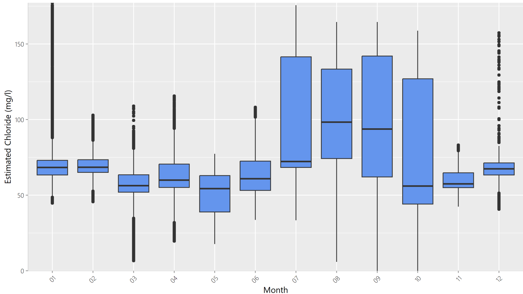
Figure A.Site16EstClBoxMonth Monthly Boxplots of Estimated Chloride at Site 16 Jackson Creek: 2018-10 to 2020-10
