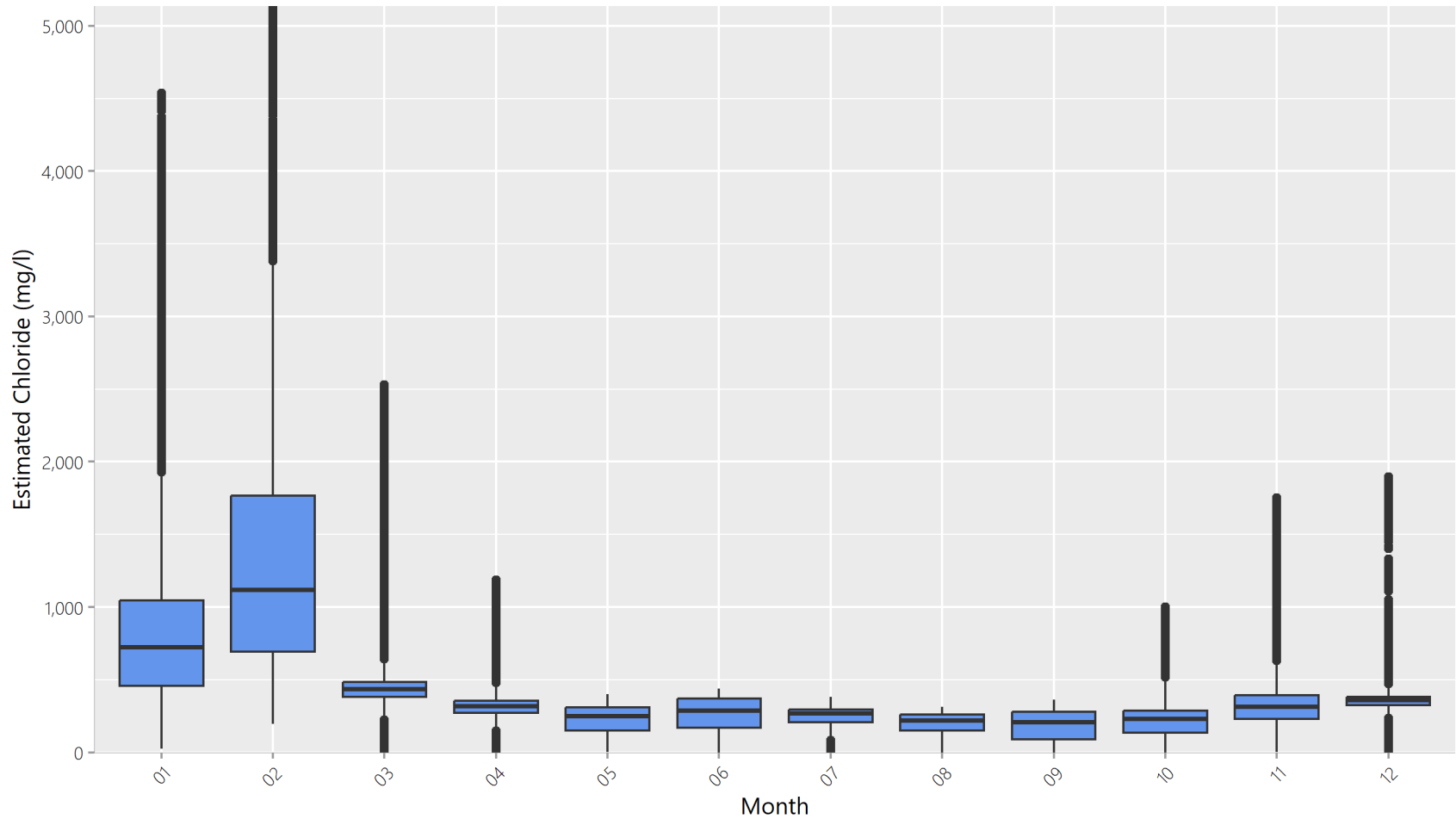
Figure A.Site12EstClBoxMonth Monthly Boxplots of Estimated Chloride at Site 12 Lincoln Creek: 2018-10 to 2021-02
