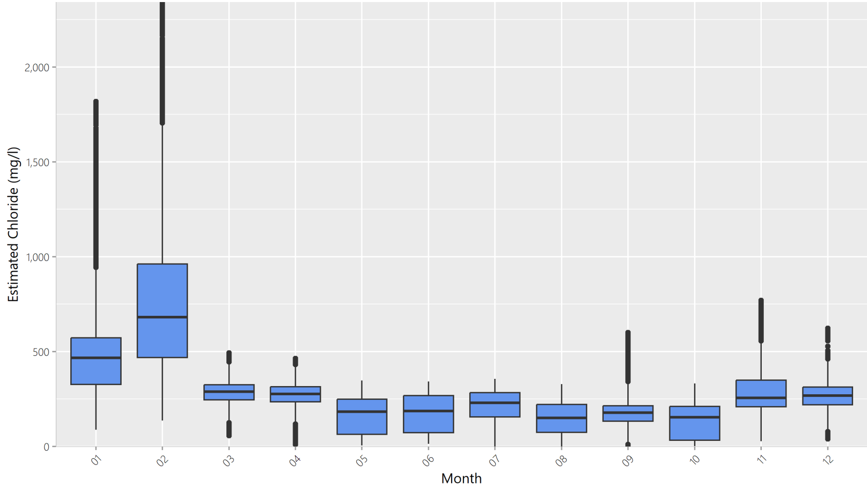
Figure A.Site09EstClBoxMonth Monthly Boxplots of Estimated Chloride at Site 09 Oak Creek: 2018-10 to 2021-02
