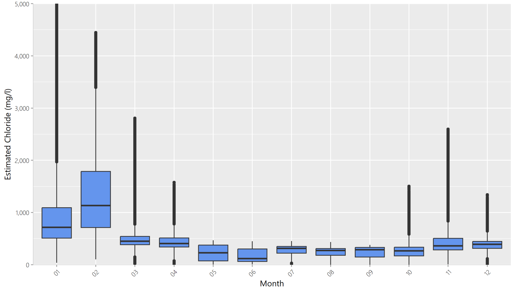
Monthly Boxplots of Estimated Chloride at Site 53 Honey Creek at Wauwatosa: 2018-10 to 2021-02
