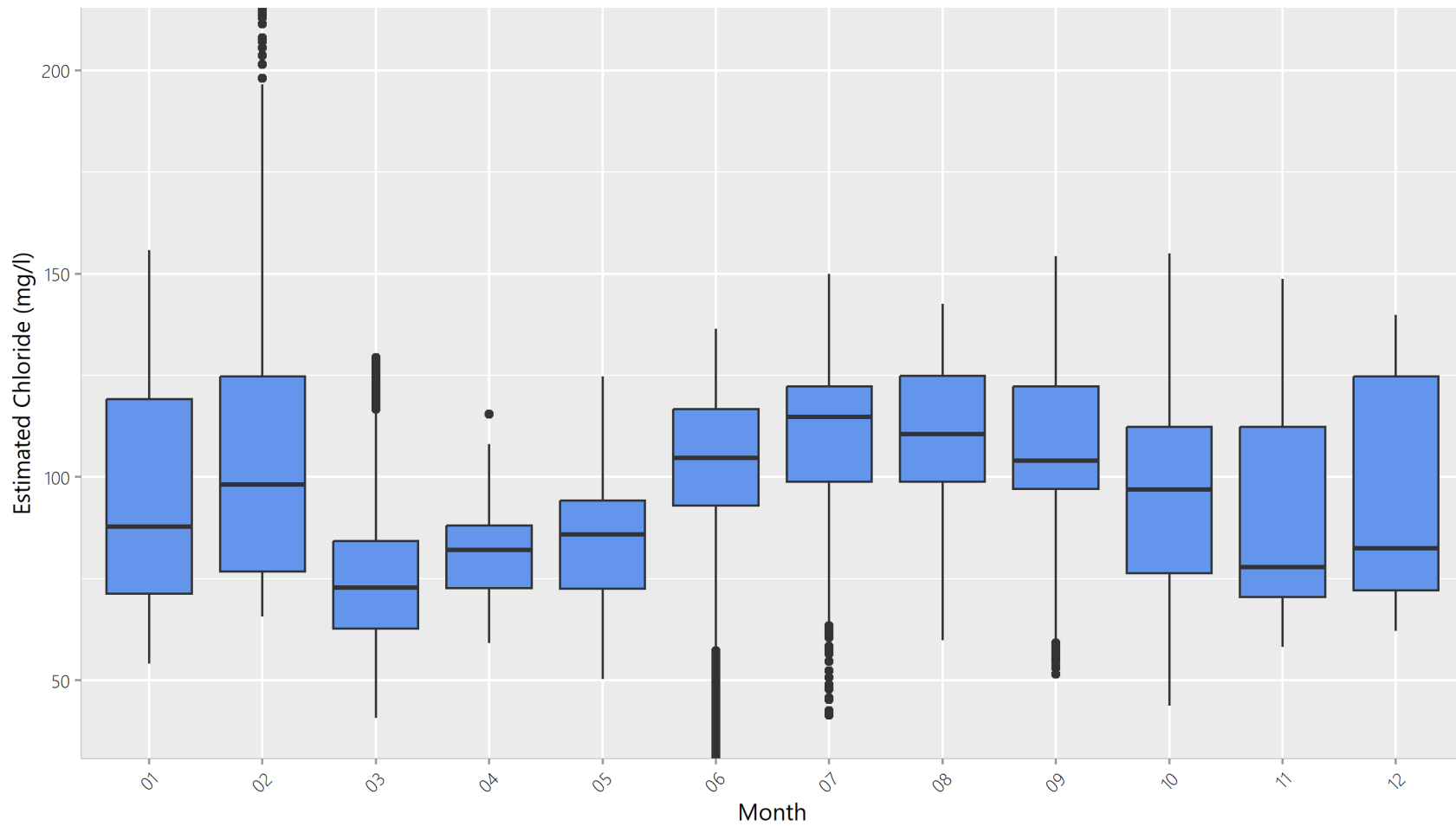
Monthly Boxplots of Estimated Chloride at Site 11 Bark River Upstream: 2018-10 to 2020-10
