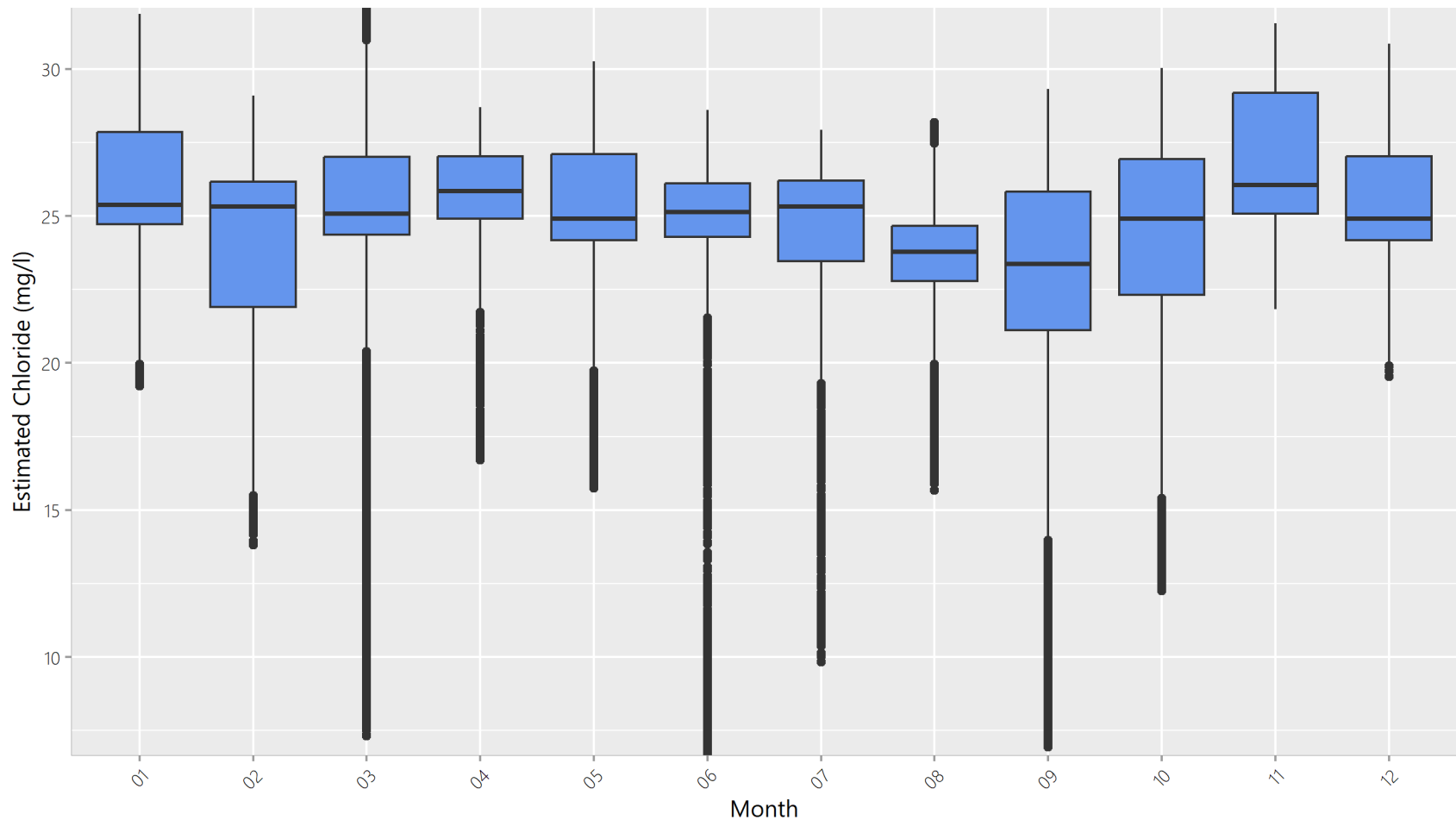
Figure A.Site54EstClBoxMonth Monthly Boxplots of Estimated Chloride at Site 54 Whitewater Creek: 2018-10 to 2020-10
