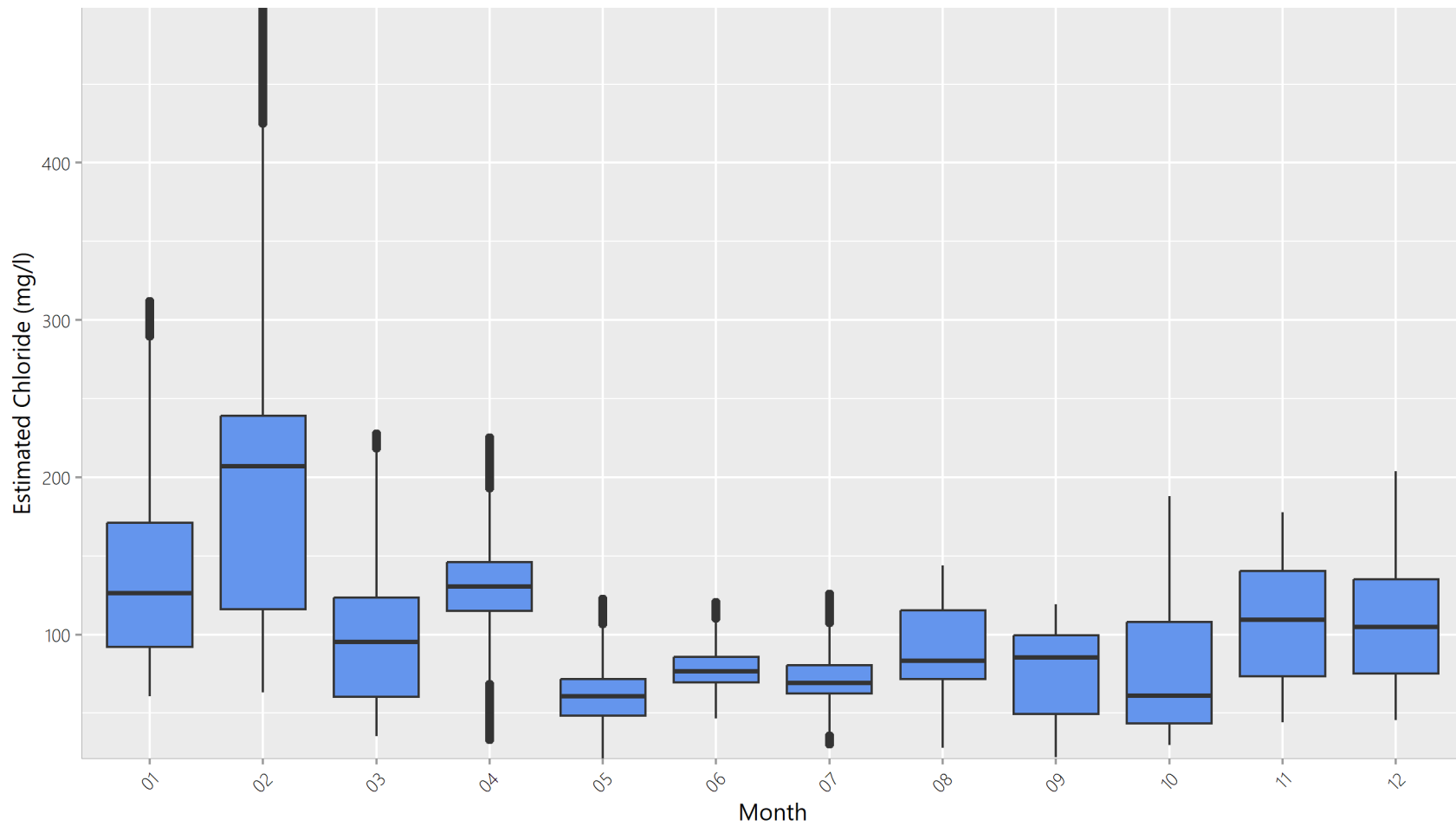
Monthly Boxplots of Estimated Chloride at Site 30 Des Plaines River: 2018-10 to 2021-02
