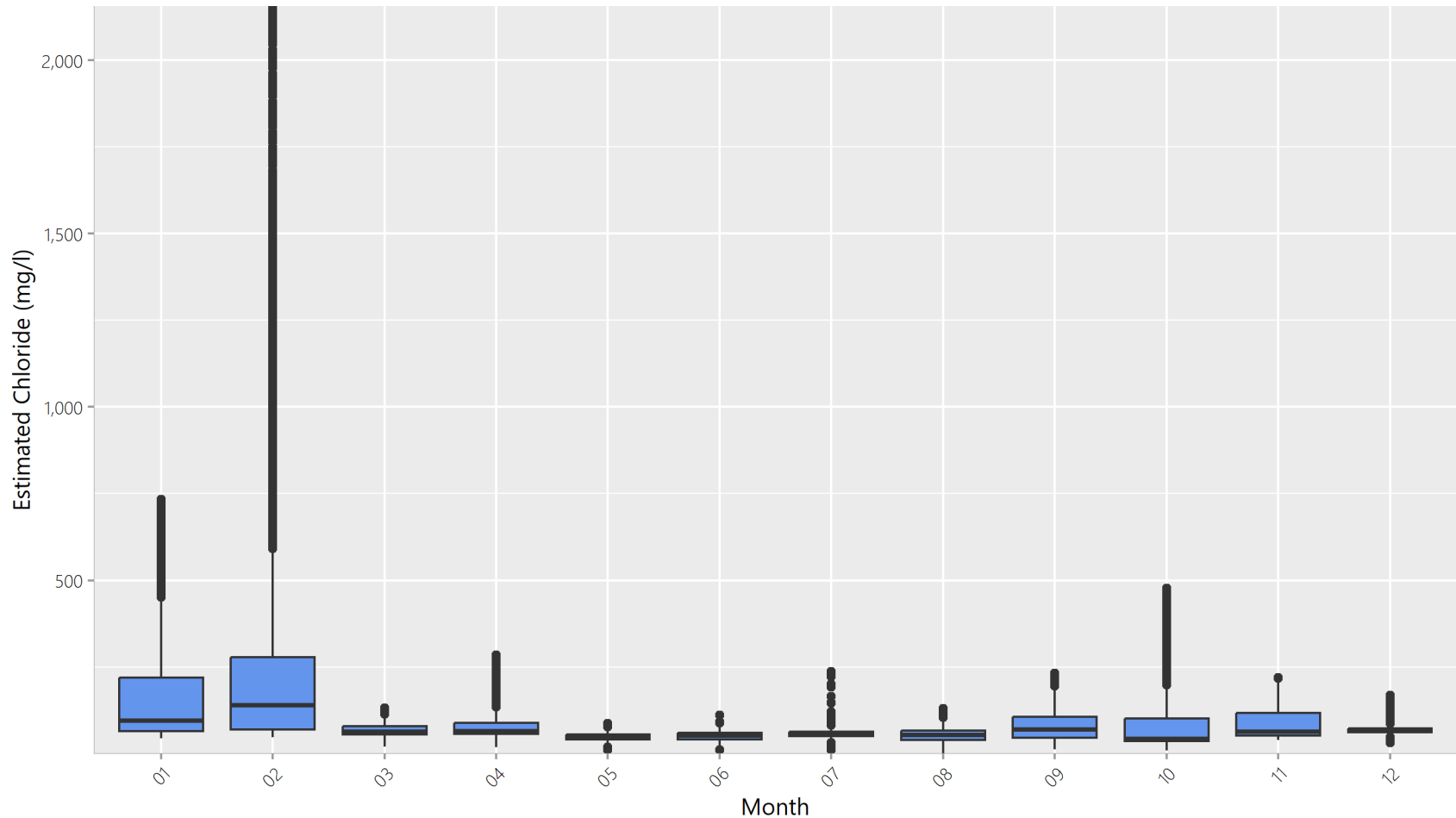
Monthly Boxplots of Estimated Chloride at Site 15 Kilbourn Road Ditch: 2018-10 to 2021-02
