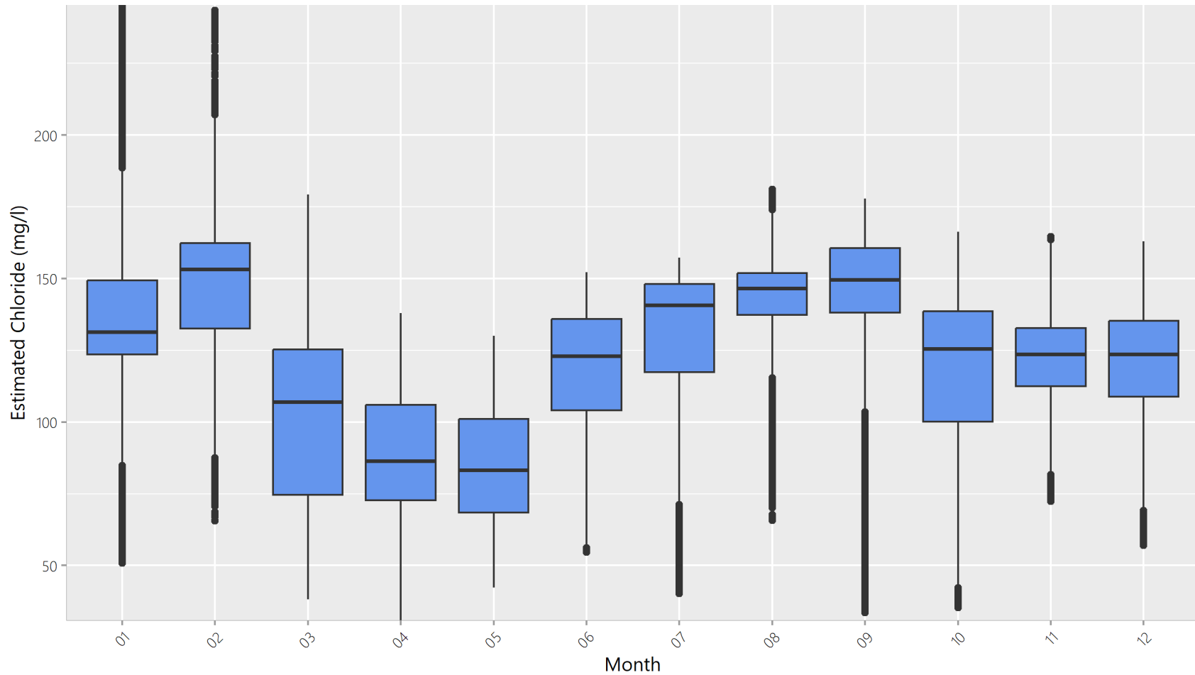
Figure A.Site33EstClBoxMonth Monthly Boxplots of Estimated Chloride at Site 33 Pebble Brook: 2018-10 to 2020-10
