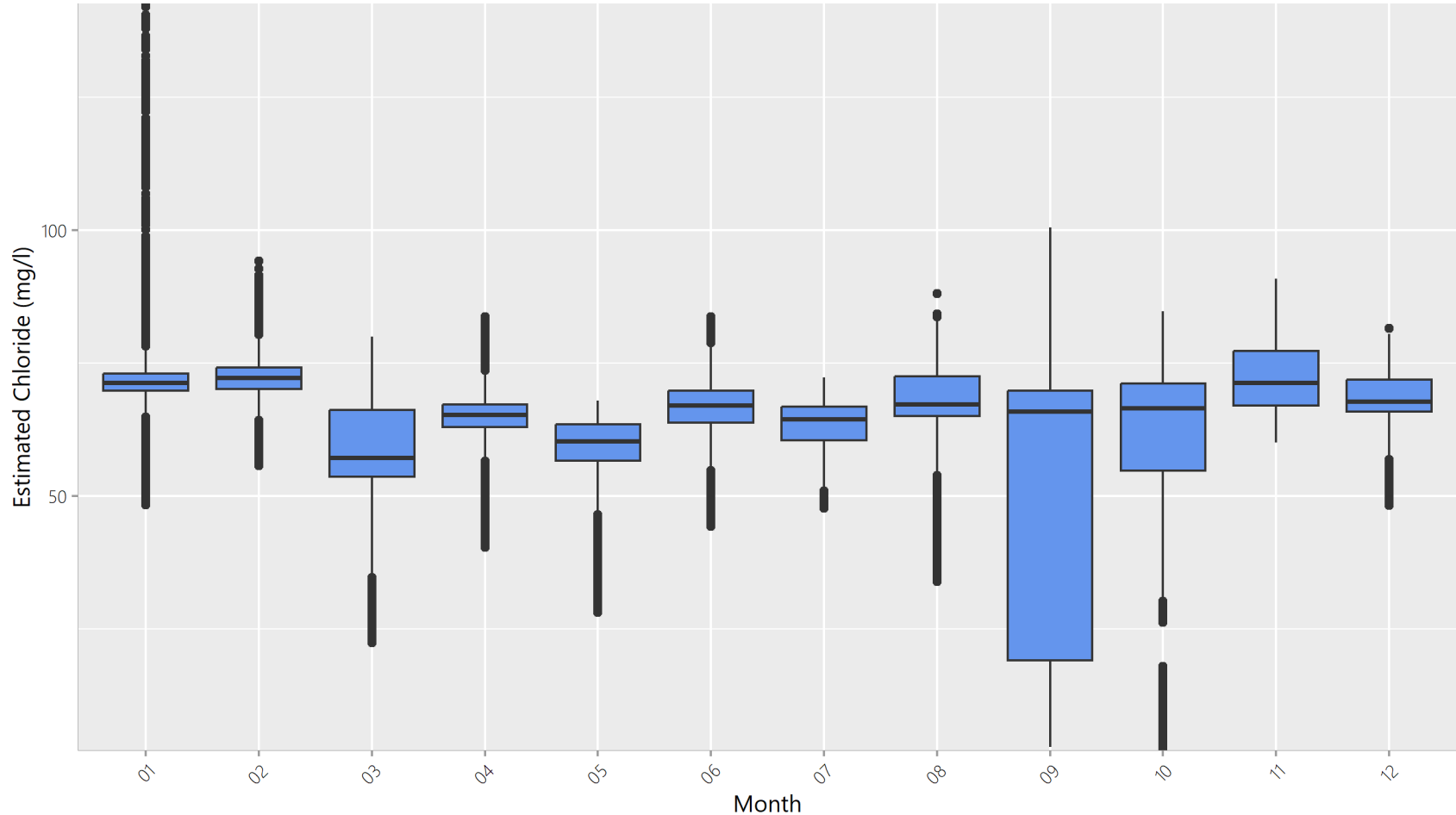
Figure A.Site06EstClBoxMonth Monthly Boxplots of Estimated Chloride at Site 06 White River near Burlington: 2018-10 to 2020-10
