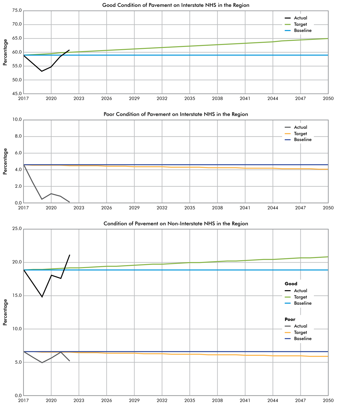
Figure P.5 Comparison of Actual Data and Targets for the National Highway System (NHS) Pavement Performance Measures
