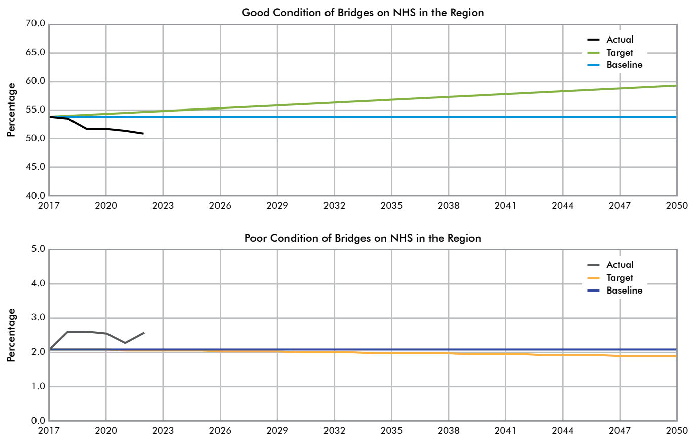
Figure P.7 Comparison of Actual Data and Targets for the National Highway System (NHS) Bridge Performance Measures
