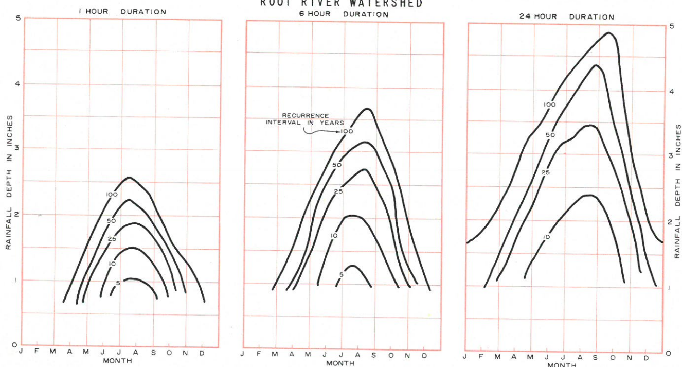
Figure 4 SEASONAL VARIATION OF RAINFALL FREQUENCY ROOT RIVER WATERSHED
