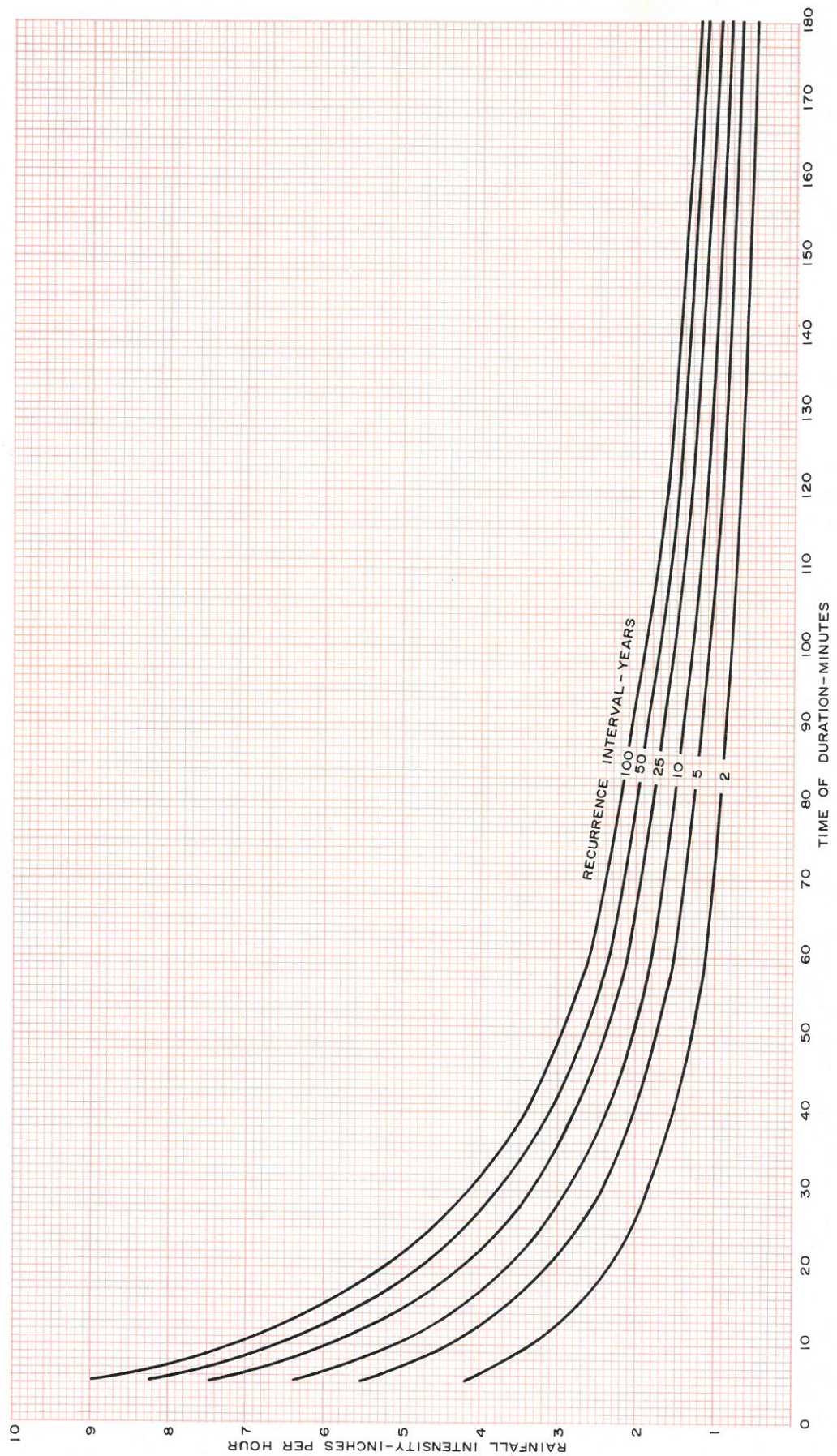
Figure 2 POINT RAINFALL INTENSITY - DURATION - FREQUENCY MILWAUKEE, WISCONSIN 1903 TO 1951
